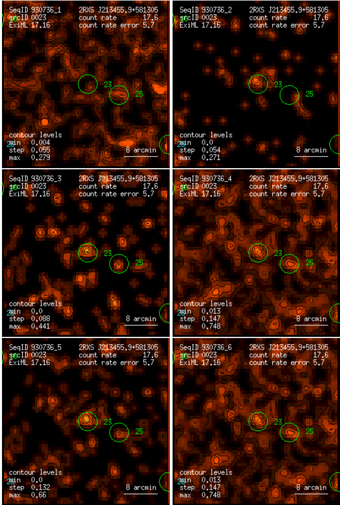
Figure 23: RASS 930736: detection 0023: band rate images, Gaussian filter: (1) PSPC channels 11 – 41, (2) 52 – 90, (3) 91 – 201, (4) 11 – 235, (5) 52 – 201, (6) 11 – 201. Broad band rates in counts/ks. Band rate contour levels in counts/ks/arcmin 2 .
