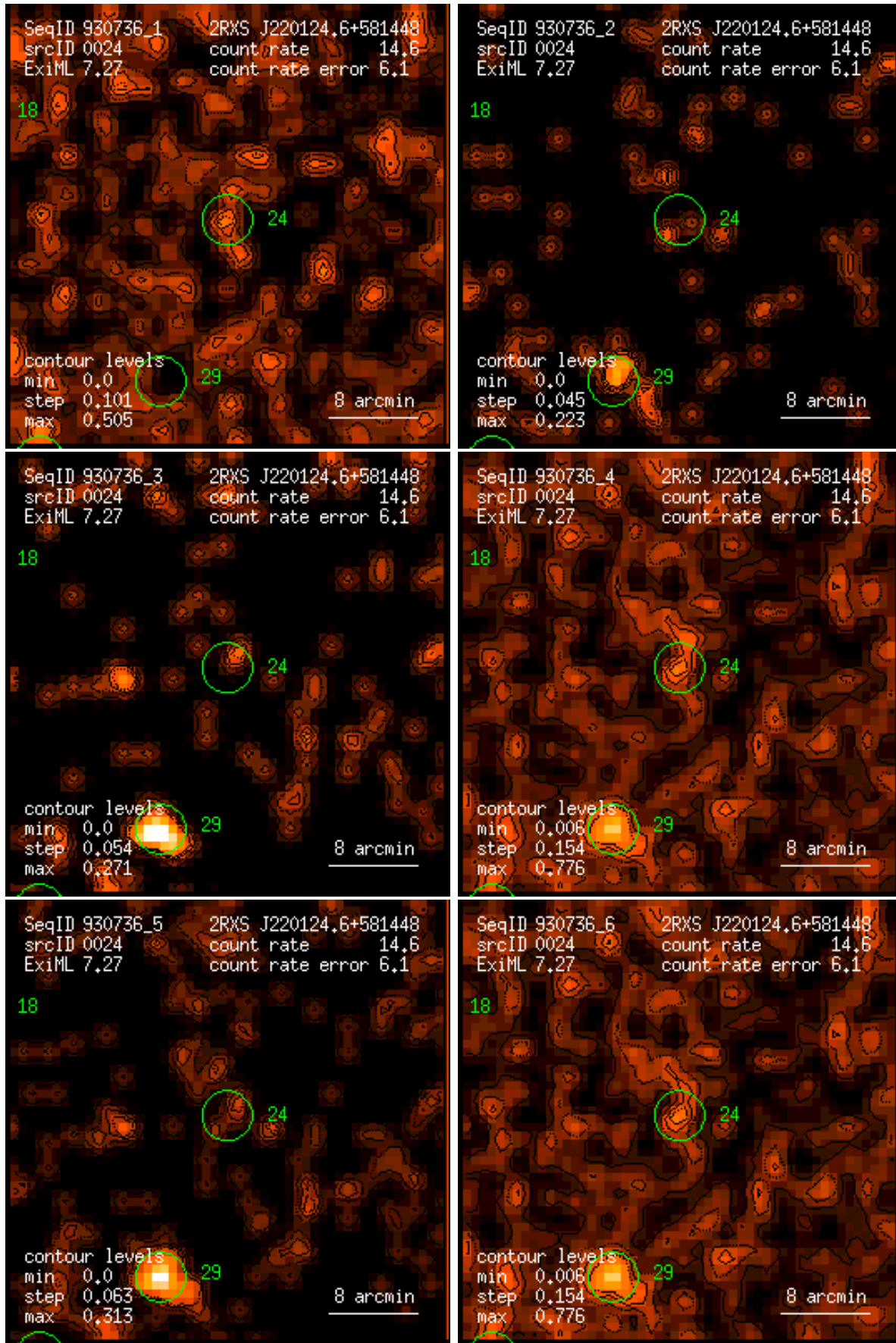
Figure 24: RASS 930736: detection 0024: band rate images, Gaussian filter: (1) PSPC channels 11 – 41, (2) 52 – 90, (3) 91 – 201, (4) 11 – 235, (5) 52 – 201, (6) 11 – 201. Broad band rates in counts/ks. Band rate contour levels in counts/ks/arcmin 2 .
