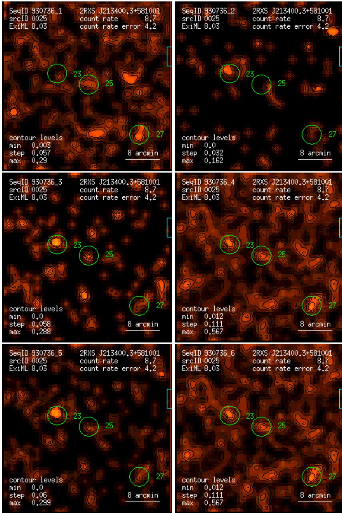
Figure 25: RASS 930736: detection 0025: band rate images, Gaussian filter: (1) PSPC channels 11 – 41, (2) 52 – 90, (3) 91 – 201, (4) 11 – 235, (5) 52 – 201, (6) 11 – 201. Broad band rates in counts/ks. Band rate contour levels in counts/ks/arcmin 2 .
