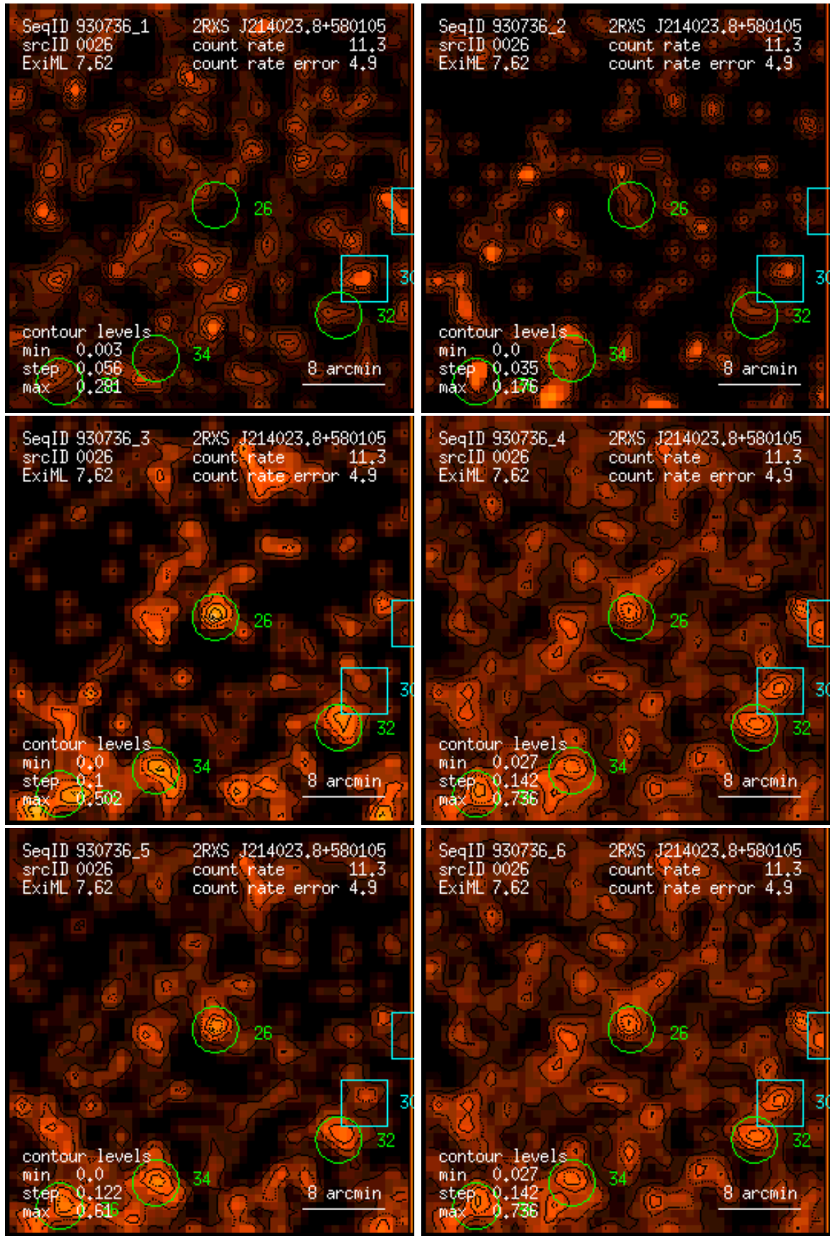
Figure 26: RASS 930736: detection 0026: band rate images, Gaussian filter: (1) PSPC channels 11 – 41, (2) 52 – 90, (3) 91 – 201, (4) 11 – 235, (5) 52 – 201, (6) 11 – 201. Broad band rates in counts/ks. Band rate contour levels in counts/ks/arcmin 2 .
