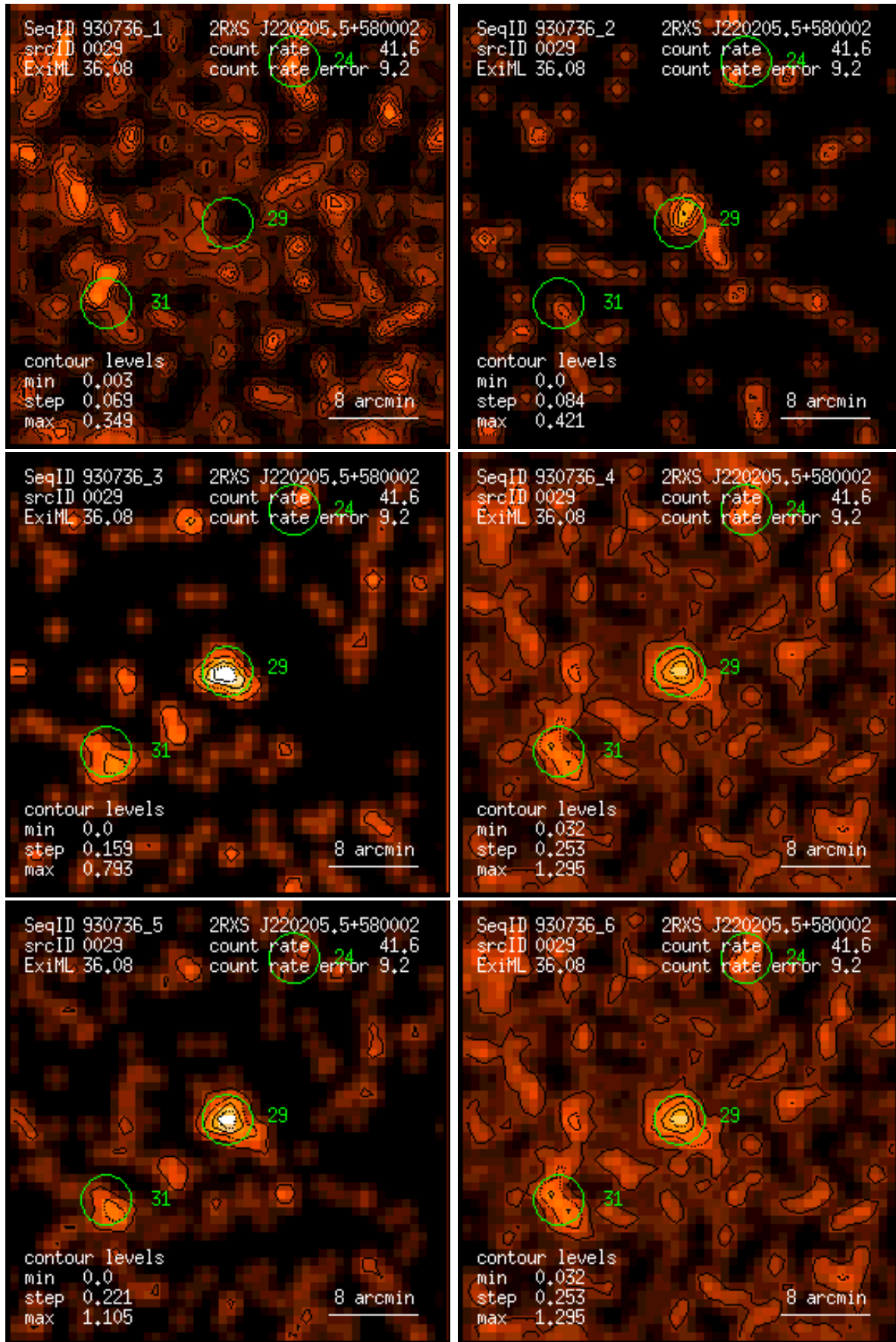
Figure 29: RASS 930736: detection 0029: band rate images, Gaussian filter: (1) PSPC channels 11 – 41, (2) 52 – 90, (3) 91 – 201, (4) 11 – 235, (5) 52 – 201, (6) 11 – 201. Broad band rates in counts/ks. Band rate contour levels in counts/ks/arcmin 2 .
