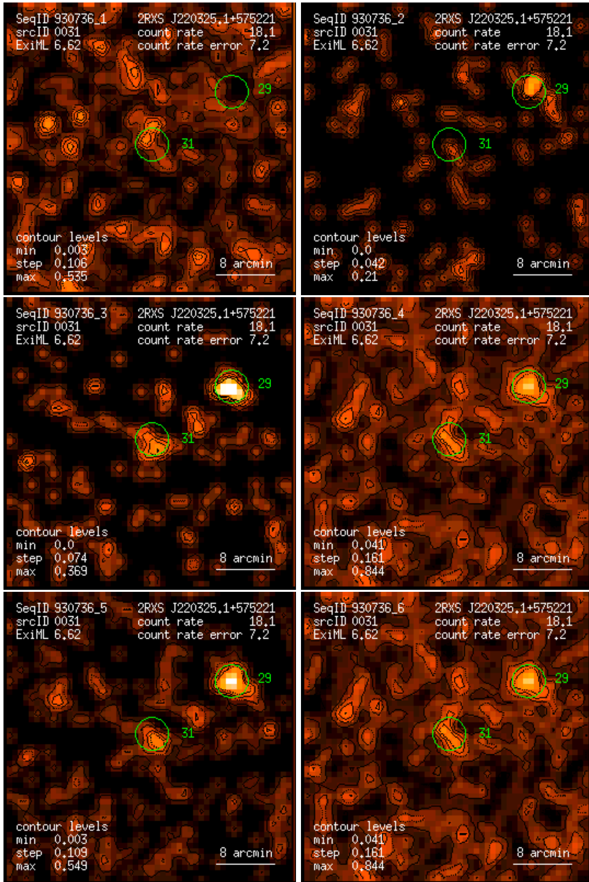
Figure 31: RASS 930736: detection 0031: band rate images, Gaussian filter: (1) PSPC channels 11 – 41, (2) 52 – 90, (3) 91 – 201, (4) 11 – 235, (5) 52 – 201, (6) 11 – 201. Broad band rates in counts/ks. Band rate contour levels in counts/ks/arcmin 2 .
