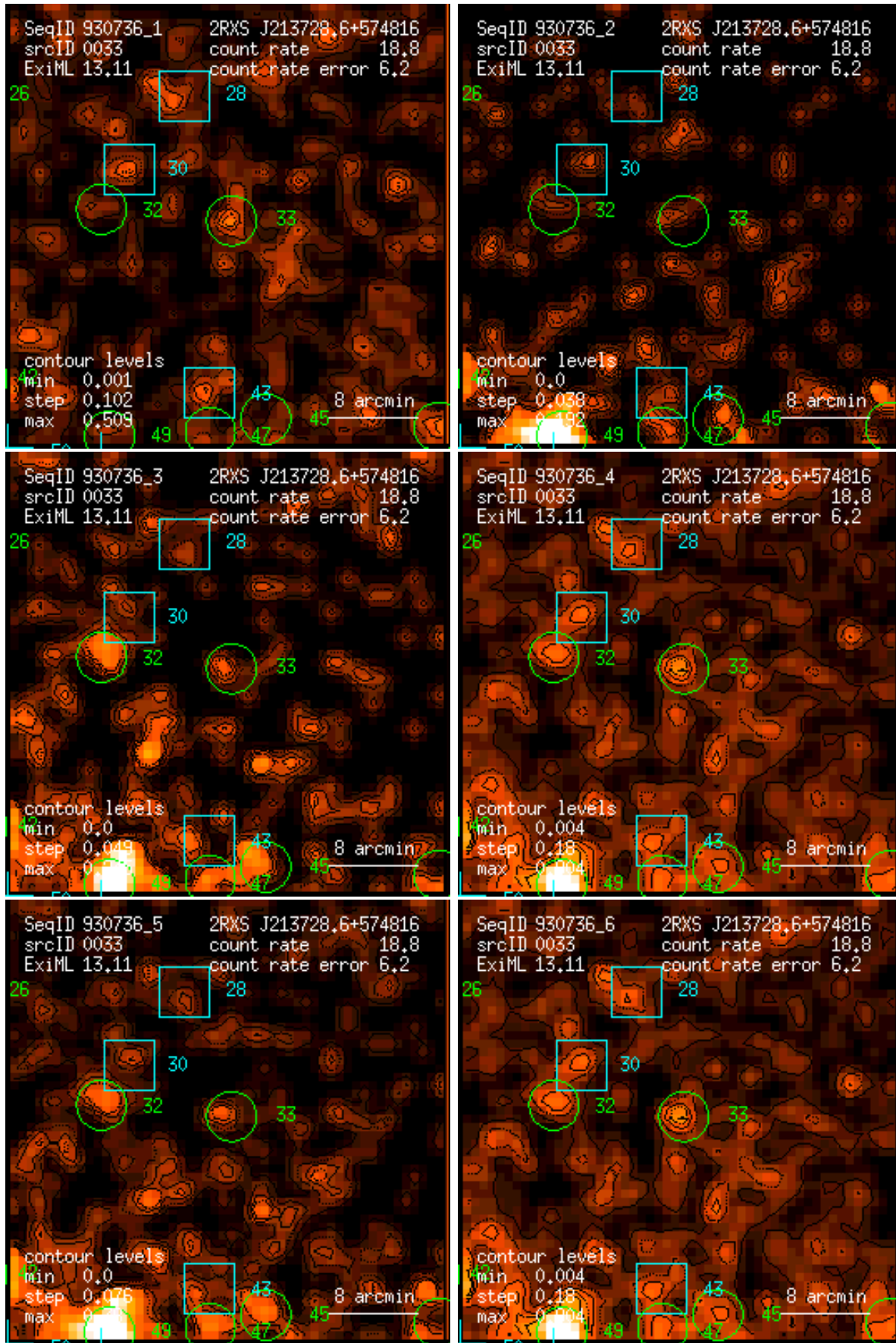
Figure 33: RASS 930736: detection 0033: band rate images, Gaussian filter: (1) PSPC channels 11 – 41, (2) 52 – 90, (3) 91 – 201, (4) 11 – 235, (5) 52 – 201, (6) 11 – 201. Broad band rates in counts/ks. Band rate contour levels in counts/ks/arcmin 2 .
