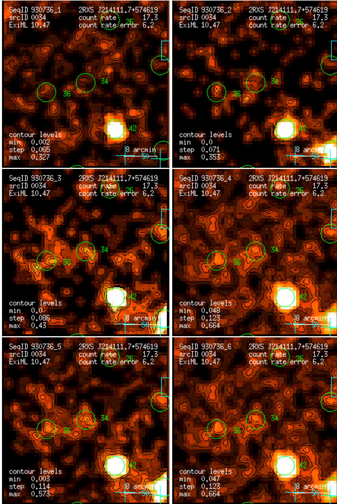
Figure 34: RASS 930736: detection 0034: band rate images, Gaussian filter: (1) PSPC channels 11 – 41, (2) 52 – 90, (3) 91 – 201, (4) 11 – 235, (5) 52 – 201, (6) 11 – 201. Broad band rates in counts/ks. Band rate contour levels in counts/ks/arcmin 2 .
