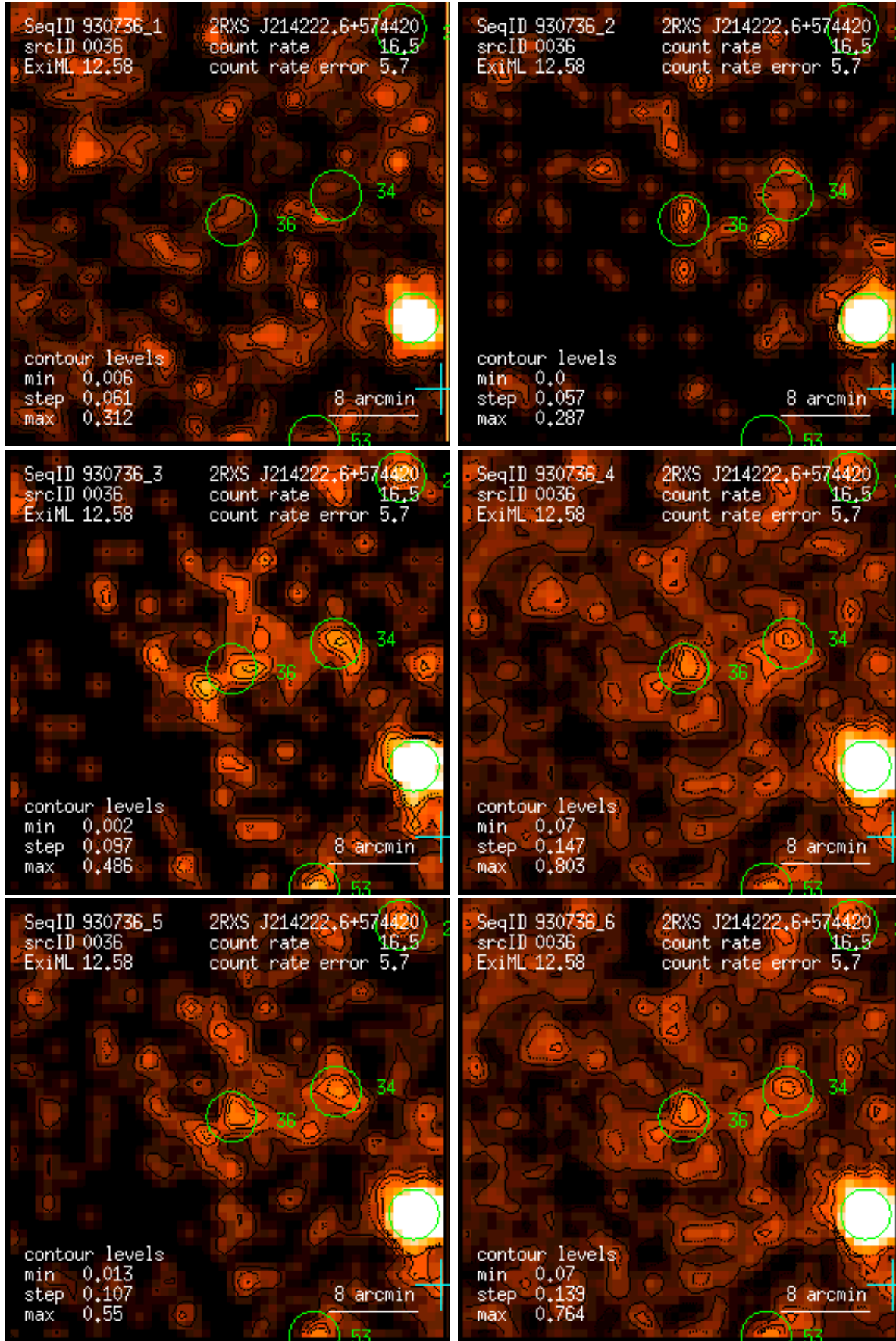
Figure 36: RASS 930736: detection 0036: band rate images, Gaussian filter: (1) PSPC channels 11 – 41, (2) 52 – 90, (3) 91 – 201, (4) 11 – 235, (5) 52 – 201, (6) 11 – 201. Broad band rates in counts/ks. Band rate contour levels in counts/ks/arcmin 2 .
