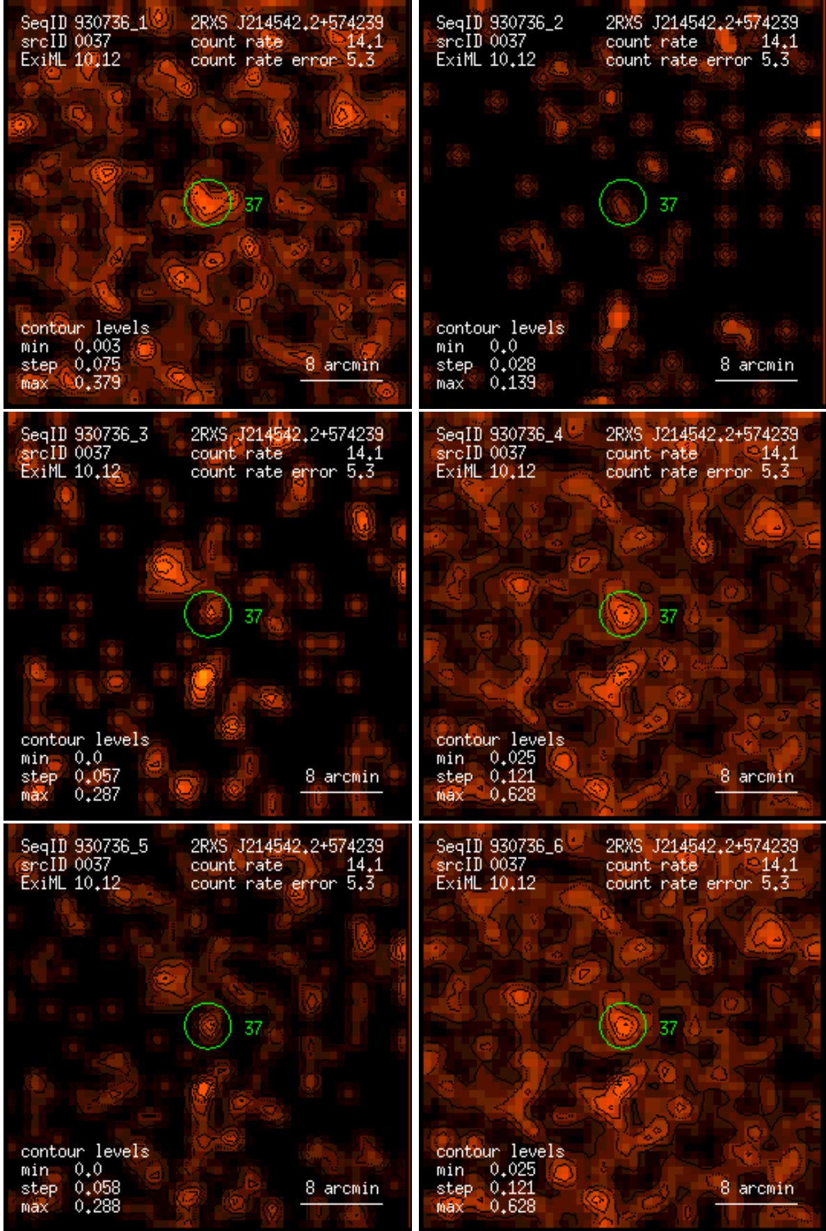
Figure 37: RASS 930736: detection 0037: band rate images, Gaussian filter: (1) PSPC channels 11 – 41, (2) 52 – 90, (3) 91 – 201, (4) 11 – 235, (5) 52 – 201, (6) 11 – 201. Broad band rates in counts/ks. Band rate contour levels in counts/ks/arcmin 2 .
