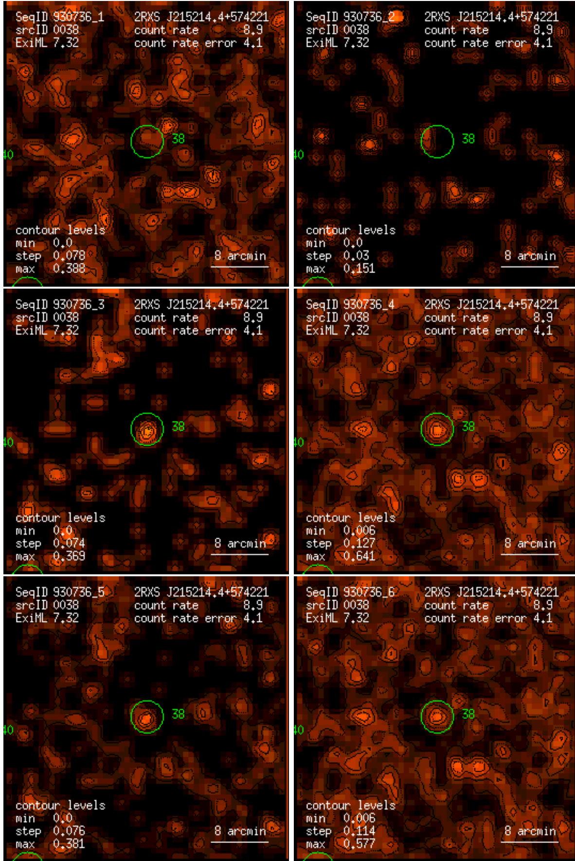
Figure 38: RASS 930736: detection 0038: band rate images, Gaussian filter: (1) PSPC channels 11 – 41, (2) 52 – 90, (3) 91 – 201, (4) 11 – 235, (5) 52 – 201, (6) 11 – 201. Broad band rates in counts/ks. Band rate contour levels in counts/ks/arcmin 2 .
