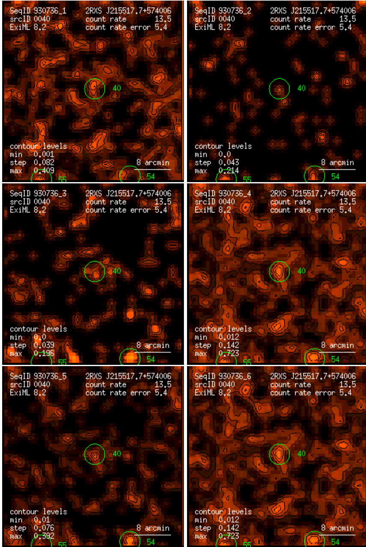
Figure 40: RASS 930736: detection 0040: band rate images, Gaussian filter: (1) PSPC channels 11 – 41, (2) 52 – 90, (3) 91 – 201, (4) 11 – 235, (5) 52 – 201, (6) 11 – 201. Broad band rates in counts/ks. Band rate contour levels in counts/ks/arcmin 2 .
