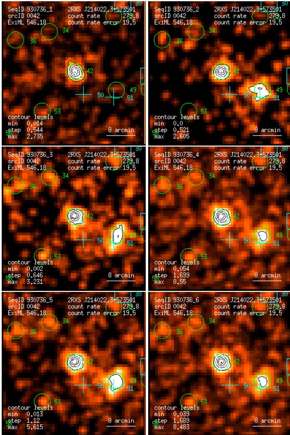
Figure 42: RASS 930736: detection 0042: band rate images, Gaussian filter: (1) PSPC channels 11 – 41, (2) 52 – 90, (3) 91 – 201, (4) 11 – 235, (5) 52 – 201, (6) 11 – 201. Broad band rates in counts/ks. Band rate contour levels in counts/ks/arcmin 2 .
