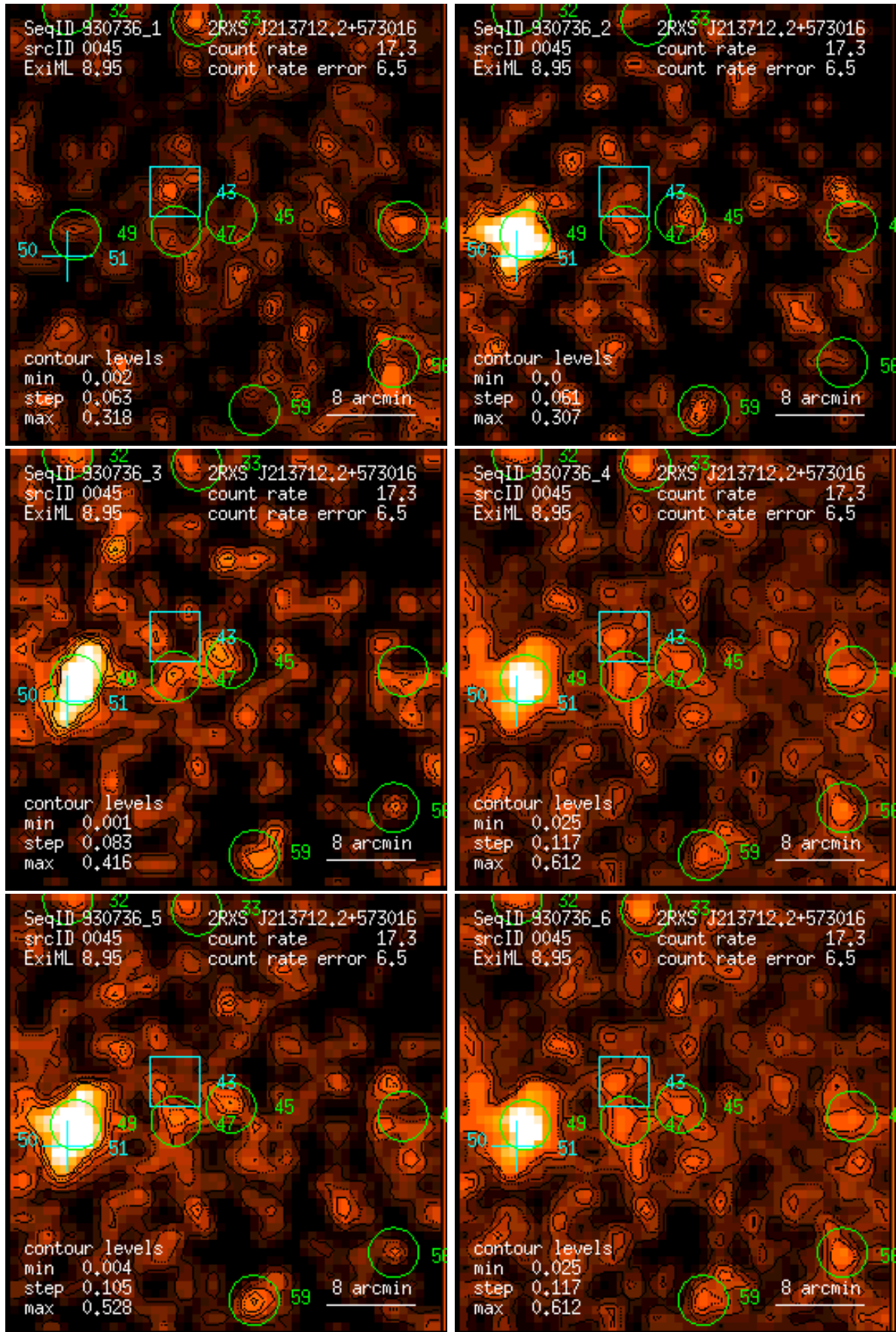
Figure 45: RASS 930736: detection 0045: band rate images, Gaussian filter: (1) PSPC channels 11 – 41, (2) 52 – 90, (3) 91 – 201, (4) 11 – 235, (5) 52 – 201, (6) 11 – 201. Broad band rates in counts/ks. Band rate contour levels in counts/ks/arcmin 2 .
