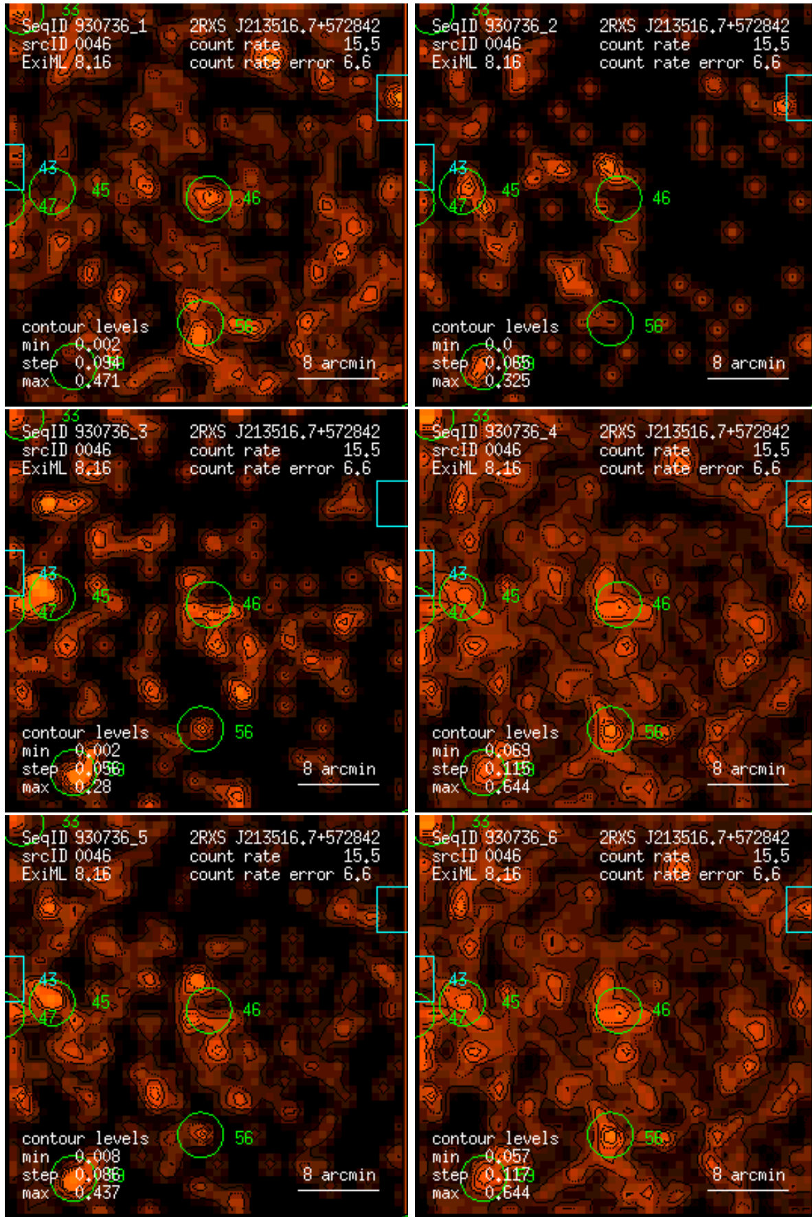
Figure 46: RASS 930736: detection 0046: band rate images, Gaussian filter: (1) PSPC channels 11 – 41, (2) 52 – 90, (3) 91 – 201, (4) 11 – 235, (5) 52 – 201, (6) 11 – 201. Broad band rates in counts/ks. Band rate contour levels in counts/ks/arcmin 2 .
