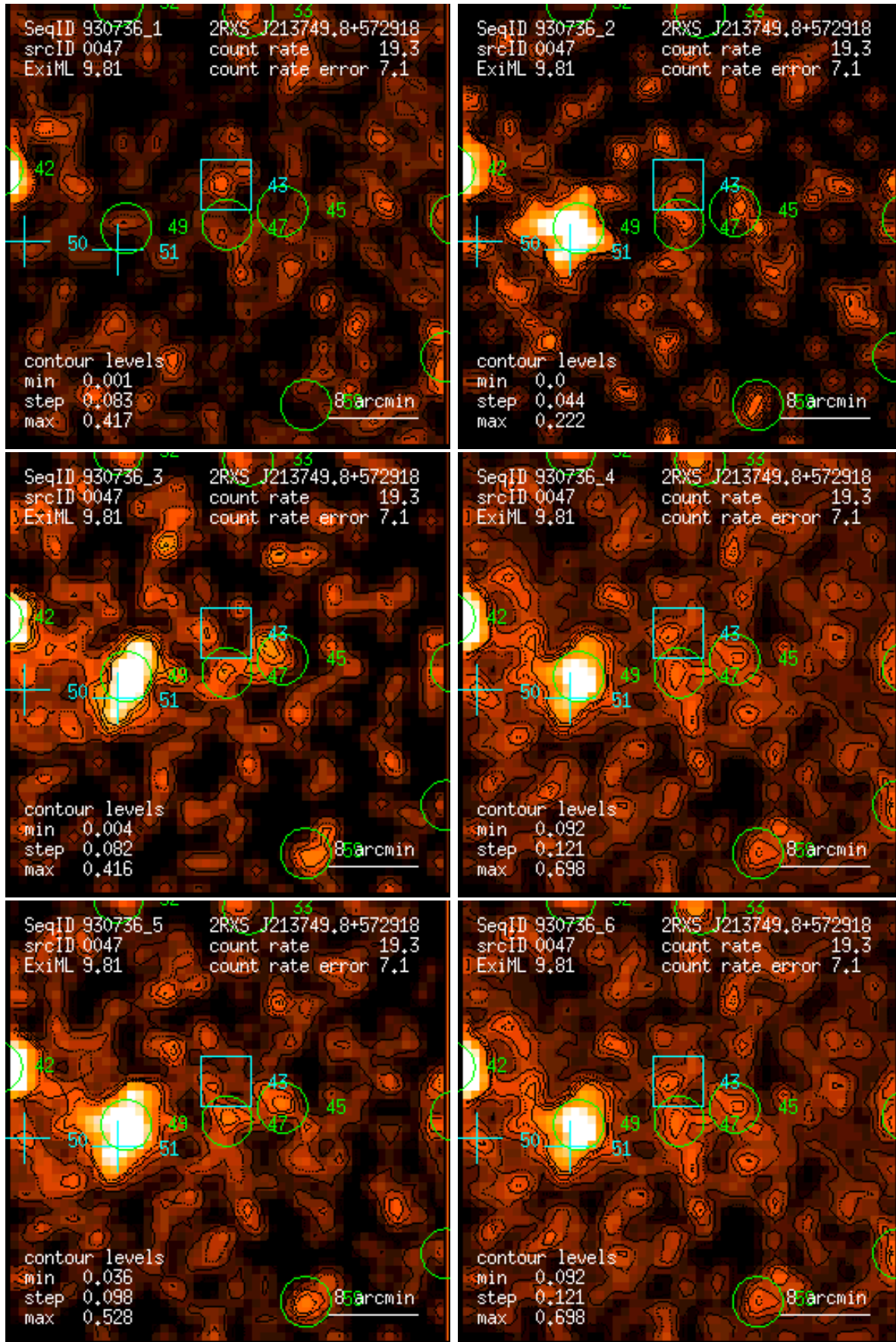
Figure 47: RASS 930736: detection 0047: band rate images, Gaussian filter: (1) PSPC channels 11 – 41, (2) 52 – 90, (3) 91 – 201, (4) 11 – 235, (5) 52 – 201, (6) 11 – 201. Broad band rates in counts/ks. Band rate contour levels in counts/ks/arcmin 2 .
