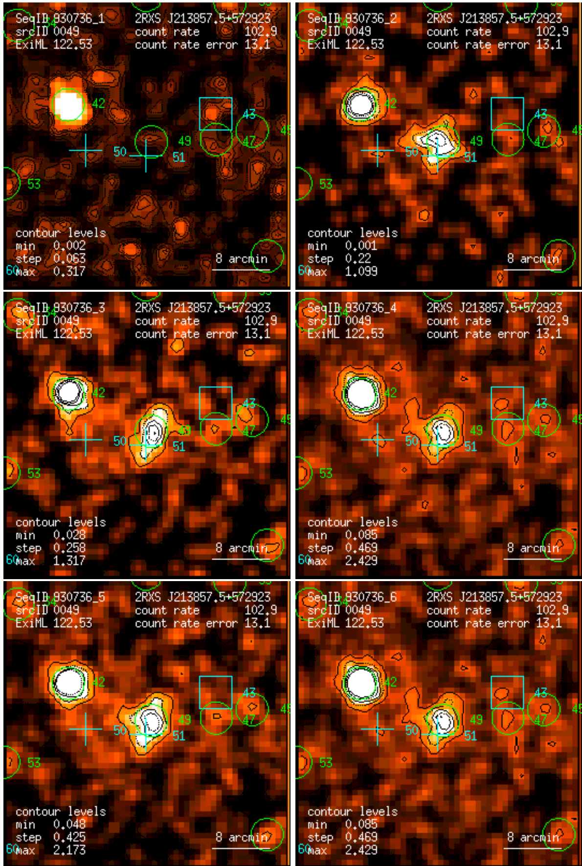
Figure 49: RASS 930736: detection 0049: band rate images, Gaussian filter: (1) PSPC channels 11 – 41, (2) 52 – 90, (3) 91 – 201, (4) 11 – 235, (5) 52 – 201, (6) 11 – 201. Broad band rates in counts/ks. Band rate contour levels in counts/ks/arcmin 2 .
