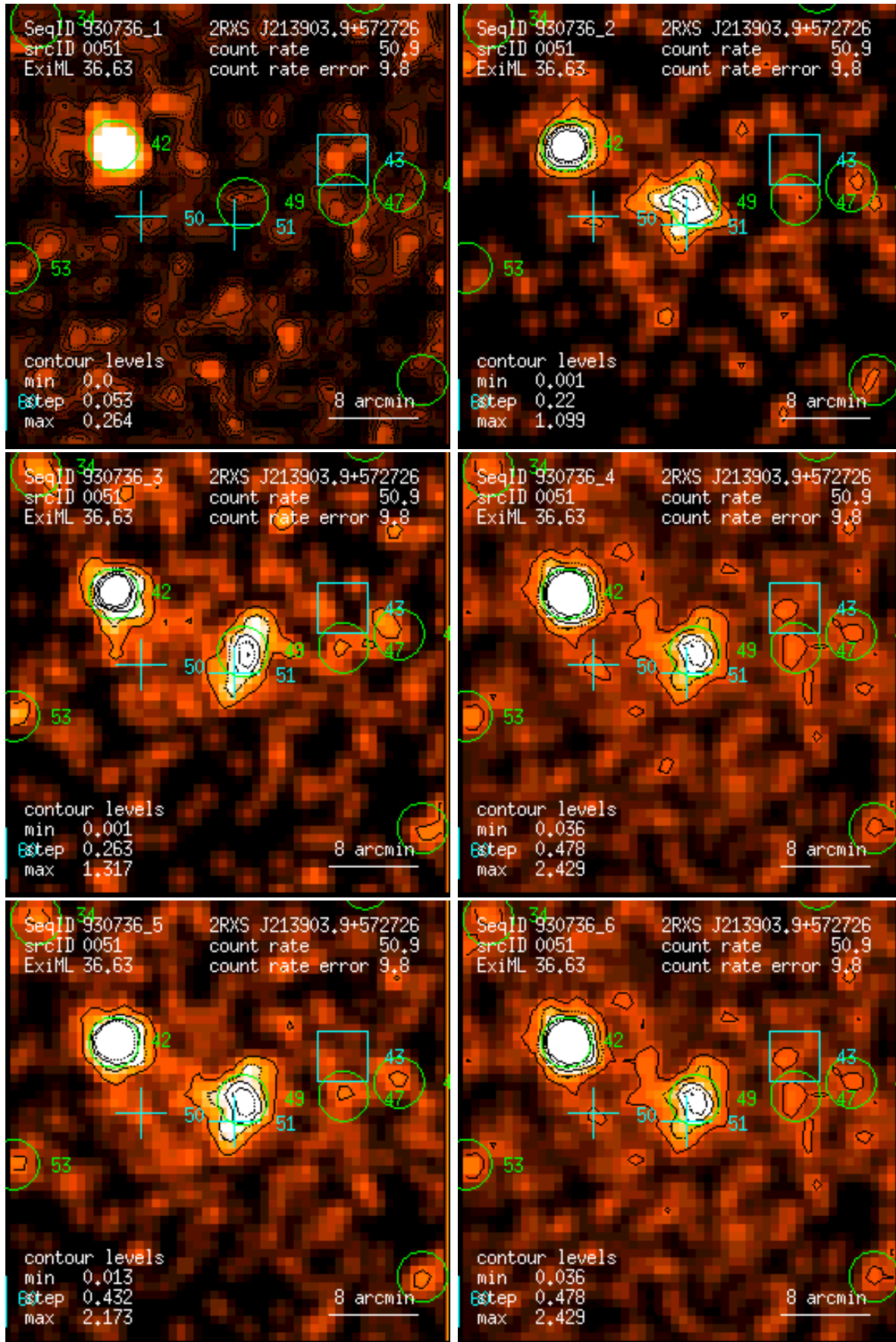
Figure 51: RASS 930736: detection 0051: band rate images, Gaussian filter: (1) PSPC channels 11 – 41, (2) 52 – 90, (3) 91 – 201, (4) 11 – 235, (5) 52 – 201, (6) 11 – 201. Broad band rates in counts/ks. Band rate contour levels in counts/ks/arcmin 2 .
