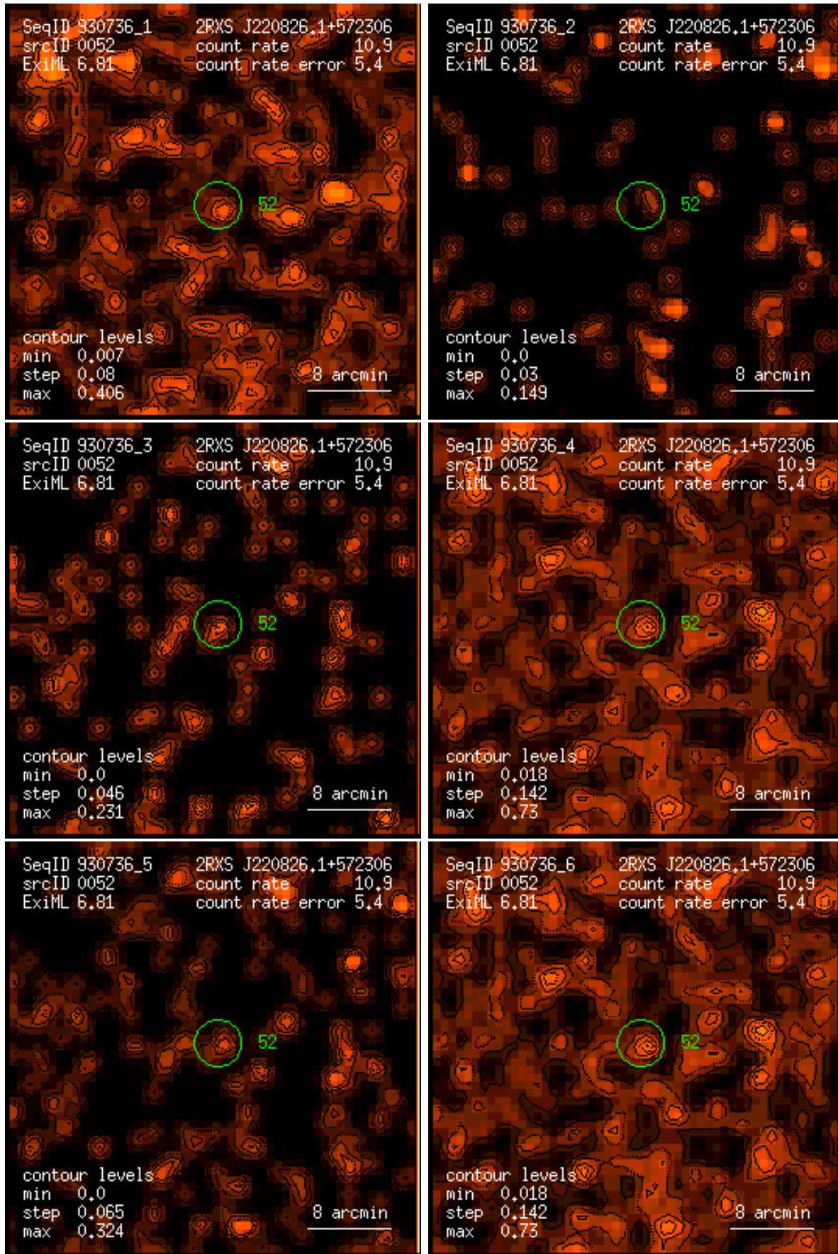
Figure 52: RASS 930736: detection 0052: band rate images, Gaussian filter: (1) PSPC channels 11 – 41, (2) 52 – 90, (3) 91 – 201, (4) 11 – 235, (5) 52 – 201, (6) 11 – 201. Broad band rates in counts/ks. Band rate contour levels in counts/ks/arcmin 2 .
