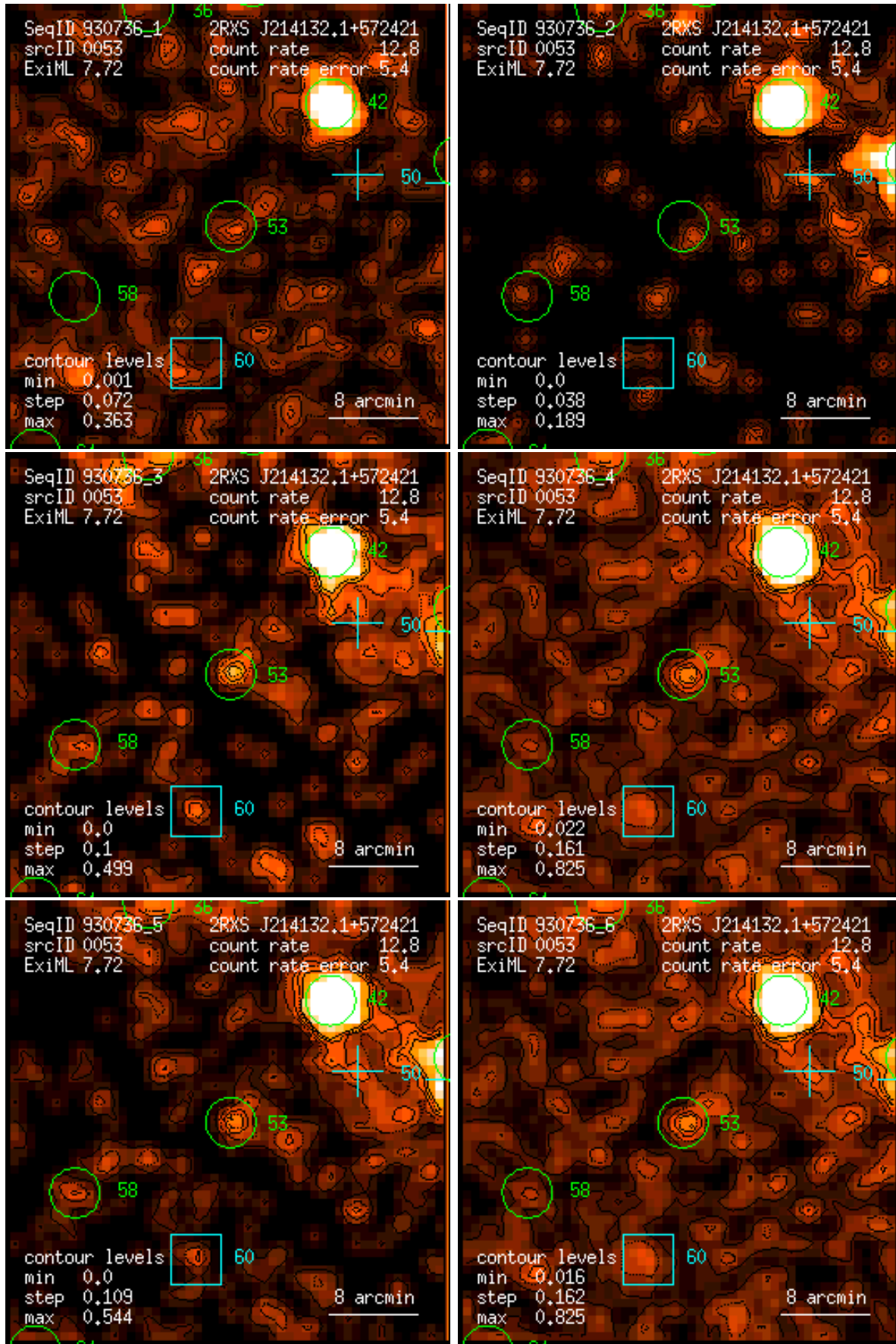
Figure 53: RASS 930736: detection 0053: band rate images, Gaussian filter: (1) PSPC channels 11 – 41, (2) 52 – 90, (3) 91 – 201, (4) 11 – 235, (5) 52 – 201, (6) 11 – 201. Broad band rates in counts/ks. Band rate contour levels in counts/ks/arcmin 2 .
