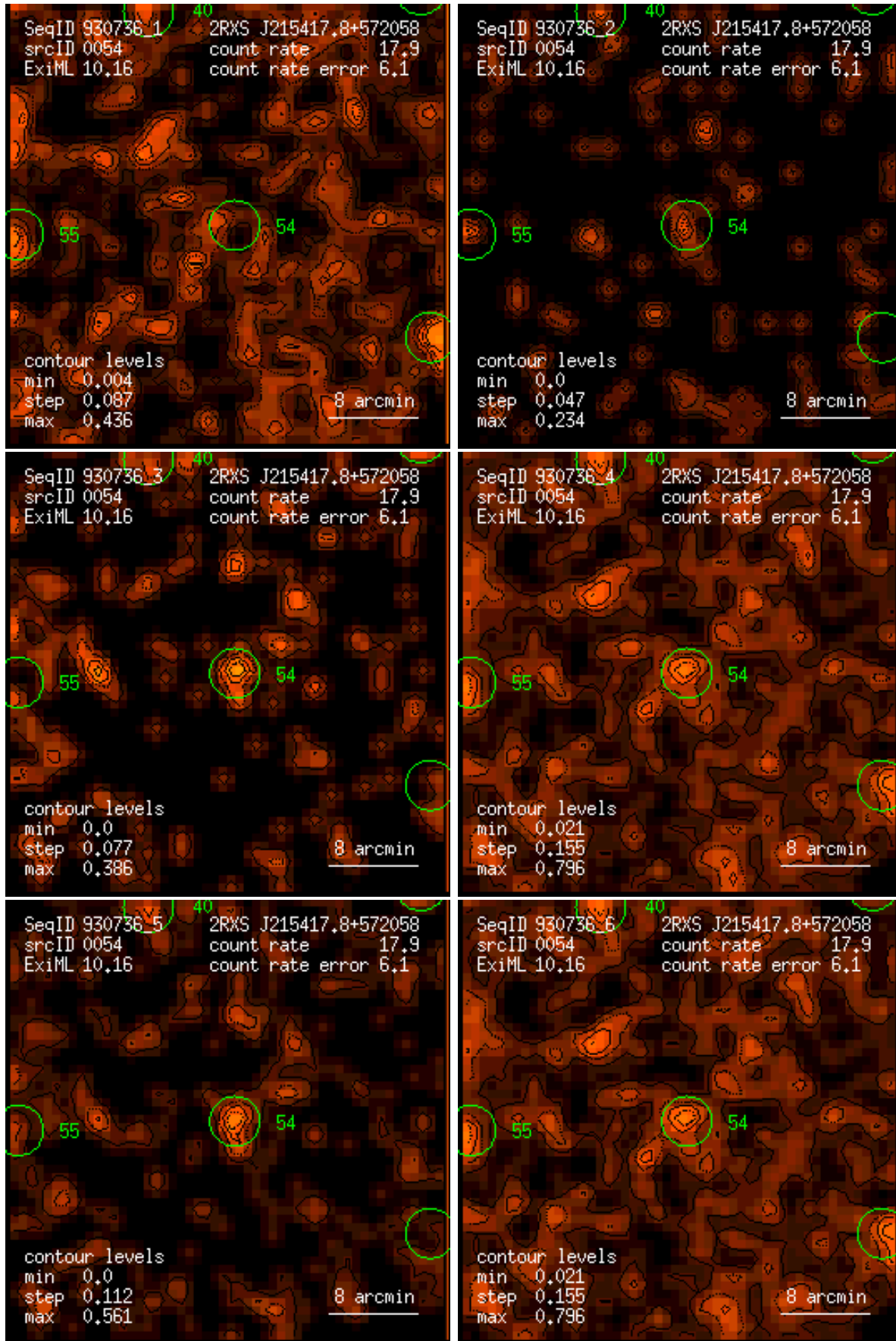
Figure 54: RASS 930736: detection 0054: band rate images, Gaussian filter: (1) PSPC channels 11 – 41, (2) 52 – 90, (3) 91 – 201, (4) 11 – 235, (5) 52 – 201, (6) 11 – 201. Broad band rates in counts/ks. Band rate contour levels in counts/ks/arcmin 2 .
