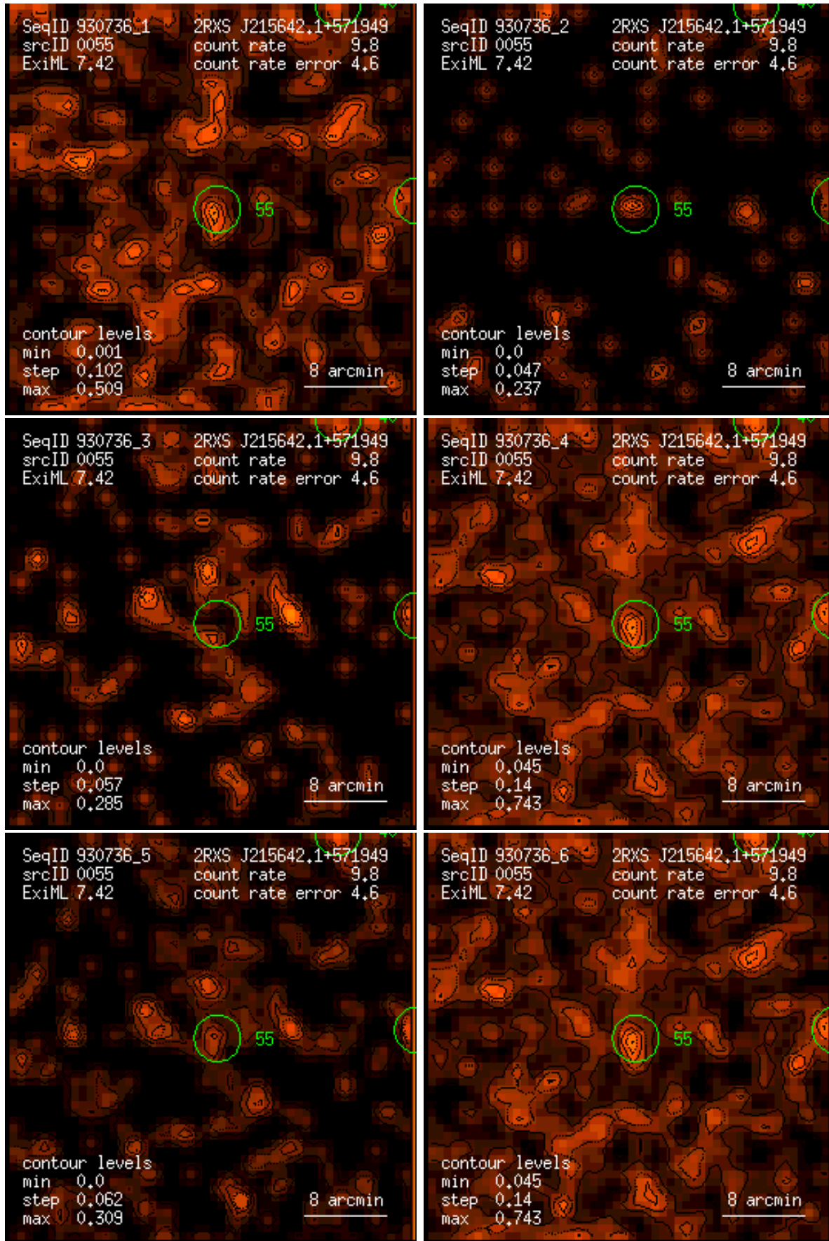
Figure 55: RASS 930736: detection 0055: band rate images, Gaussian filter: (1) PSPC channels 11 – 41, (2) 52 – 90, (3) 91 – 201, (4) 11 – 235, (5) 52 – 201, (6) 11 – 201. Broad band rates in counts/ks. Band rate contour levels in counts/ks/arcmin 2 .
