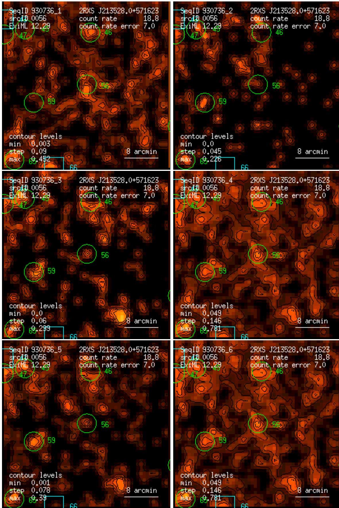
Figure 56: RASS 930736: detection 0056: band rate images, Gaussian filter: (1) PSPC channels 11 – 41, (2) 52 – 90, (3) 91 – 201, (4) 11 – 235, (5) 52 – 201, (6) 11 – 201. Broad band rates in counts/ks. Band rate contour levels in counts/ks/arcmin 2 .
