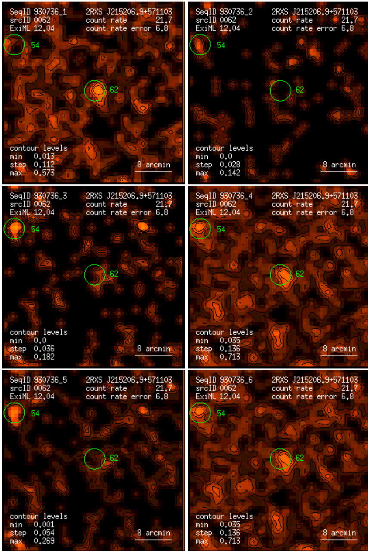
Figure 62: RASS 930736: detection 0062: band rate images, Gaussian filter: (1) PSPC channels 11 – 41, (2) 52 – 90, (3) 91 – 201, (4) 11 – 235, (5) 52 – 201, (6) 11 – 201. Broad band rates in counts/ks. Band rate contour levels in counts/ks/arcmin 2 .
