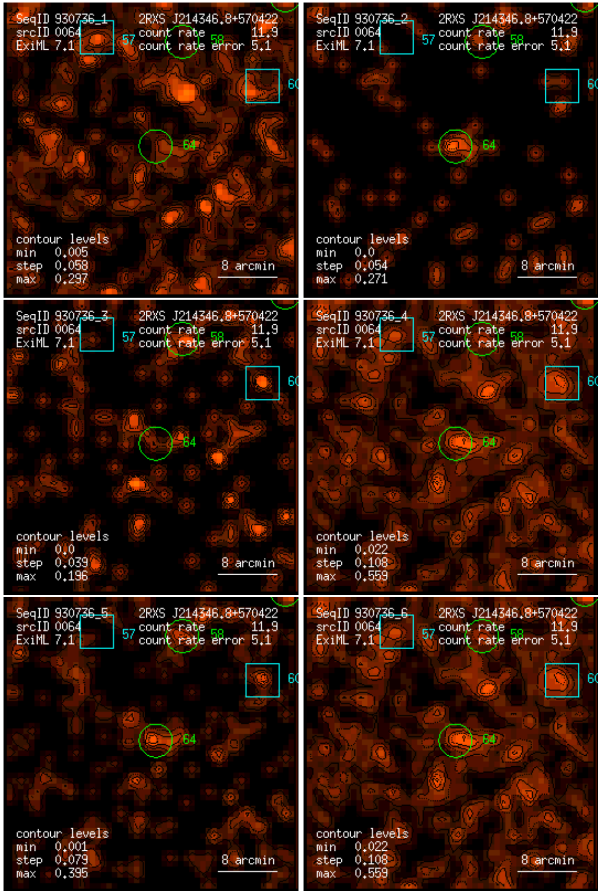
Figure 64: RASS 930736: detection 0064: band rate images, Gaussian filter: (1) PSPC channels 11 – 41, (2) 52 – 90, (3) 91 – 201, (4) 11 – 235, (5) 52 – 201, (6) 11 – 201. Broad band rates in counts/ks. Band rate contour levels in counts/ks/arcmin 2 .
