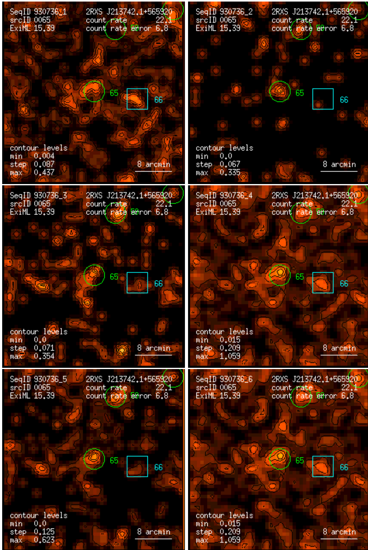
Figure 65: RASS 930736: detection 0065: band rate images, Gaussian filter: (1) PSPC channels 11 – 41, (2) 52 – 90, (3) 91 – 201, (4) 11 – 235, (5) 52 – 201, (6) 11 – 201. Broad band rates in counts/ks. Band rate contour levels in counts/ks/arcmin 2 .
