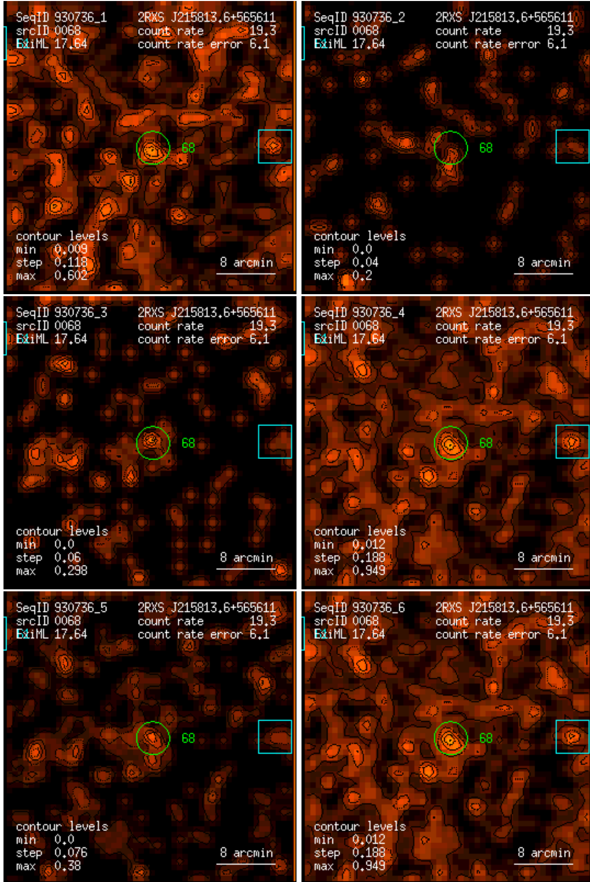
Figure 68: RASS 930736: detection 0068: band rate images, Gaussian filter: (1) PSPC channels 11 – 41, (2) 52 – 90, (3) 91 – 201, (4) 11 – 235, (5) 52 – 201, (6) 11 – 201. Broad band rates in counts/ks. Band rate contour levels in counts/ks/arcmin 2 .
