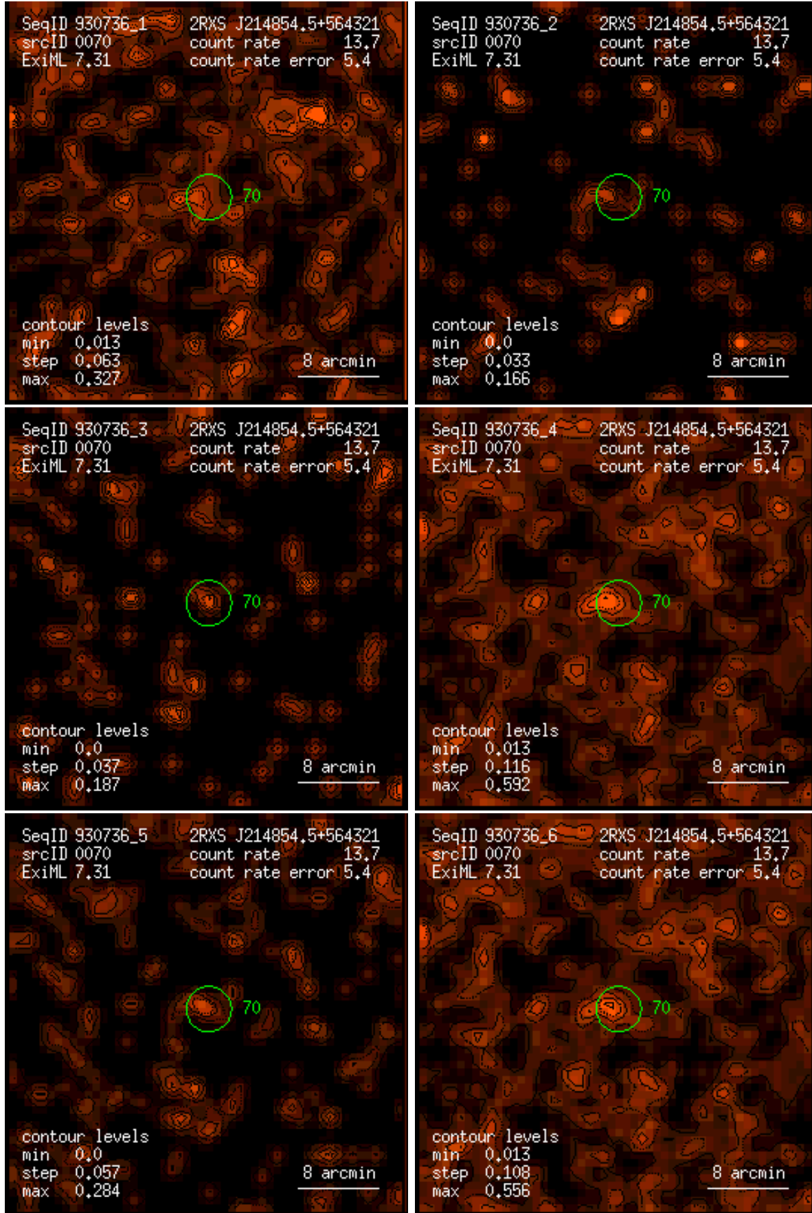
Figure 70: RASS 930736: detection 0070: band rate images, Gaussian filter: (1) PSPC channels 11 – 41, (2) 52 – 90, (3) 91 – 201, (4) 11 – 235, (5) 52 – 201, (6) 11 – 201. Broad band rates in counts/ks. Band rate contour levels in counts/ks/arcmin 2 .
