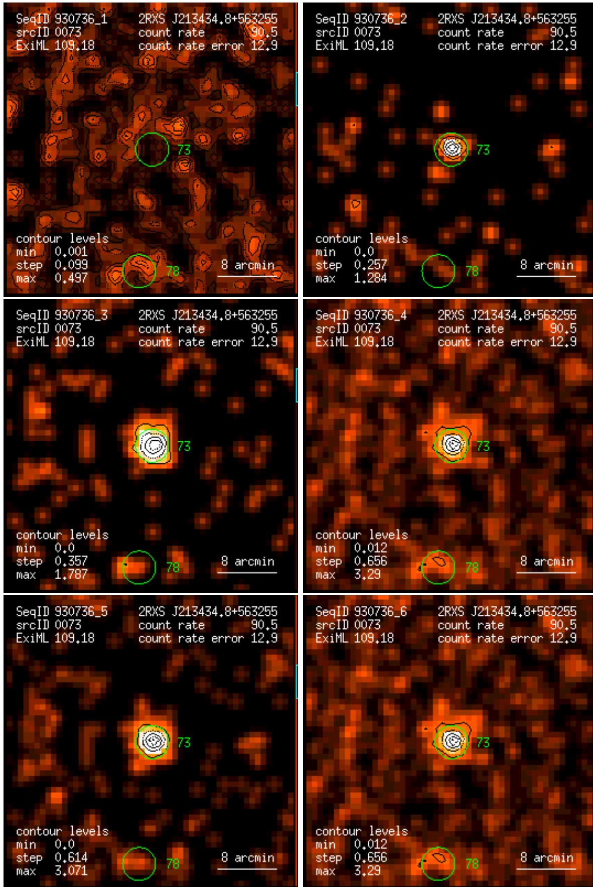
Figure 73: RASS 930736: detection 0073: band rate images, Gaussian filter: (1) PSPC channels 11 – 41, (2) 52 – 90, (3) 91 – 201, (4) 11 – 235, (5) 52 – 201, (6) 11 – 201. Broad band rates in counts/ks. Band rate contour levels in counts/ks/arcmin 2 .
