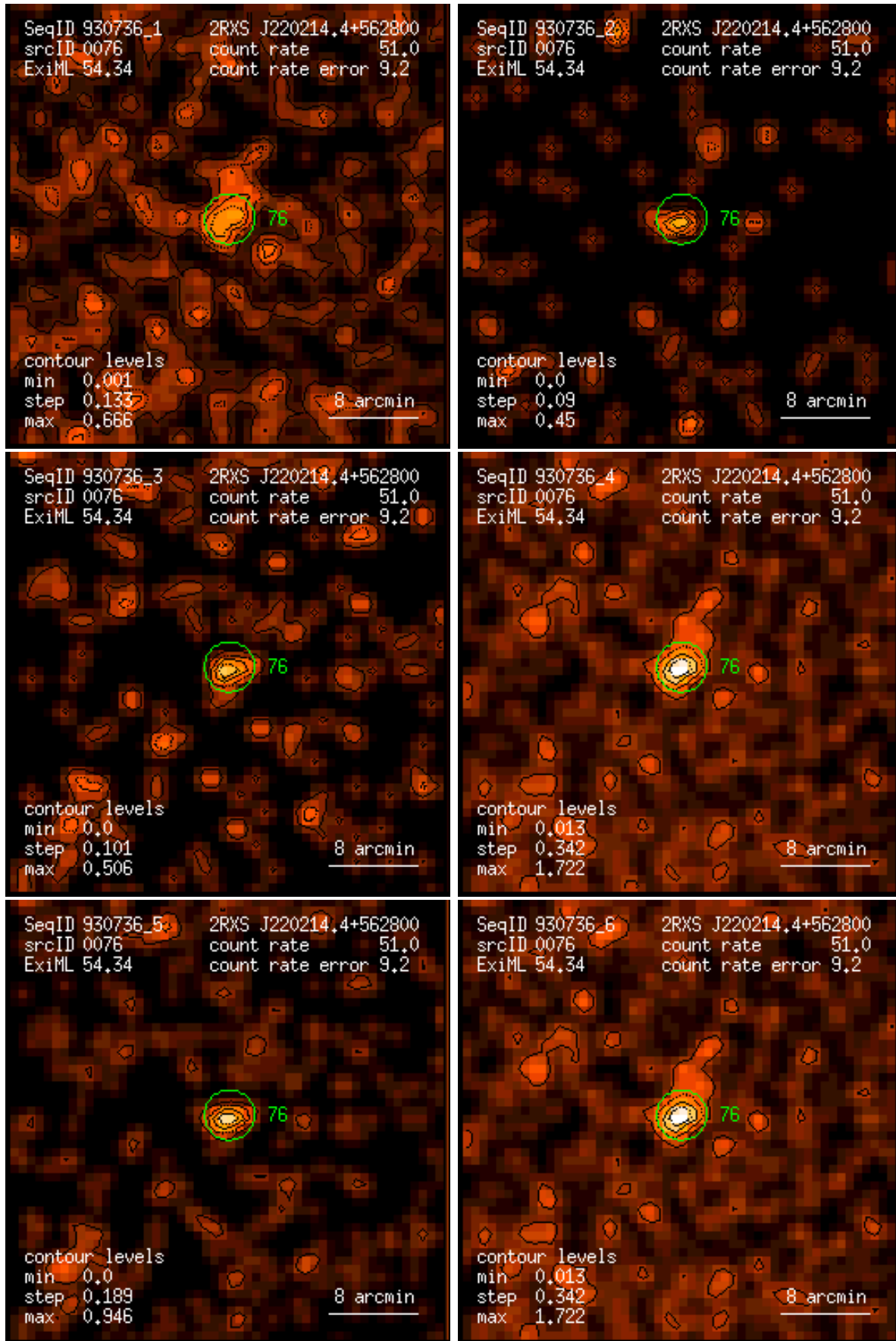
Figure 76: RASS 930736: detection 0076: band rate images, Gaussian filter: (1) PSPC channels 11 – 41, (2) 52 – 90, (3) 91 – 201, (4) 11 – 235, (5) 52 – 201, (6) 11 – 201. Broad band rates in counts/ks. Band rate contour levels in counts/ks/arcmin 2 .
