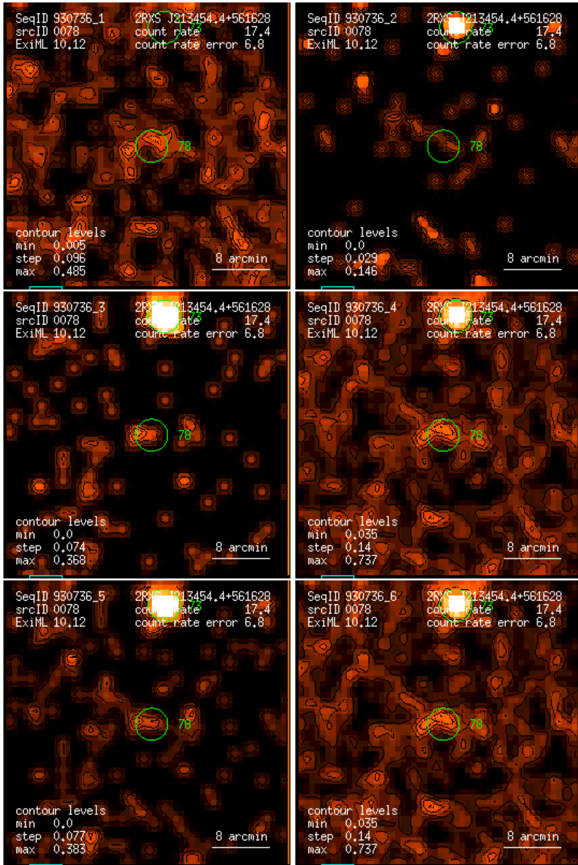
Figure 78: RASS 930736: detection 0078: band rate images, Gaussian filter: (1) PSPC channels 11 – 41, (2) 52 – 90, (3) 91 – 201, (4) 11 – 235, (5) 52 – 201, (6) 11 – 201. Broad band rates in counts/ks. Band rate contour levels in counts/ks/arcmin 2 .
