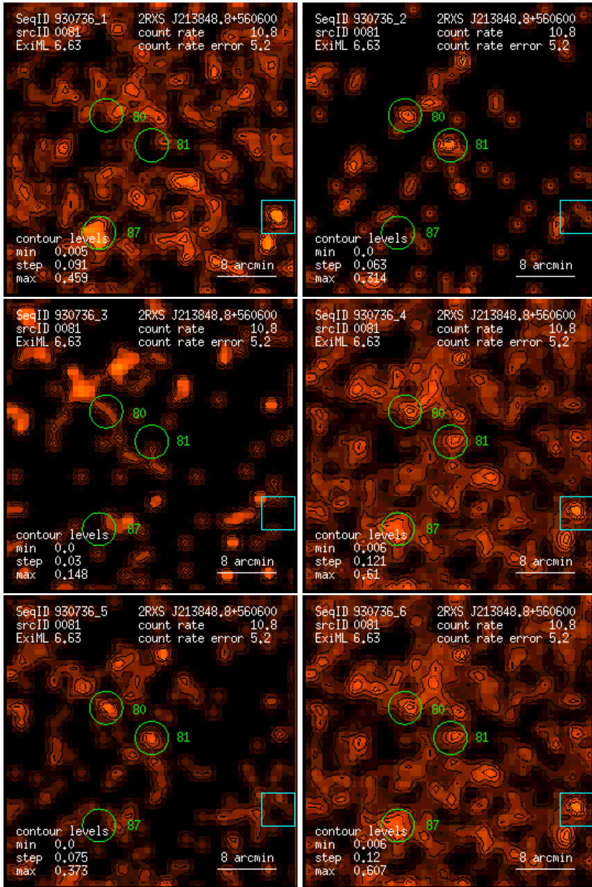
Figure 81: RASS 930736: detection 0081: band rate images, Gaussian filter: (1) PSPC channels 11 – 41, (2) 52 – 90, (3) 91 – 201, (4) 11 – 235, (5) 52 – 201, (6) 11 – 201. Broad band rates in counts/ks. Band rate contour levels in counts/ks/arcmin 2 .
