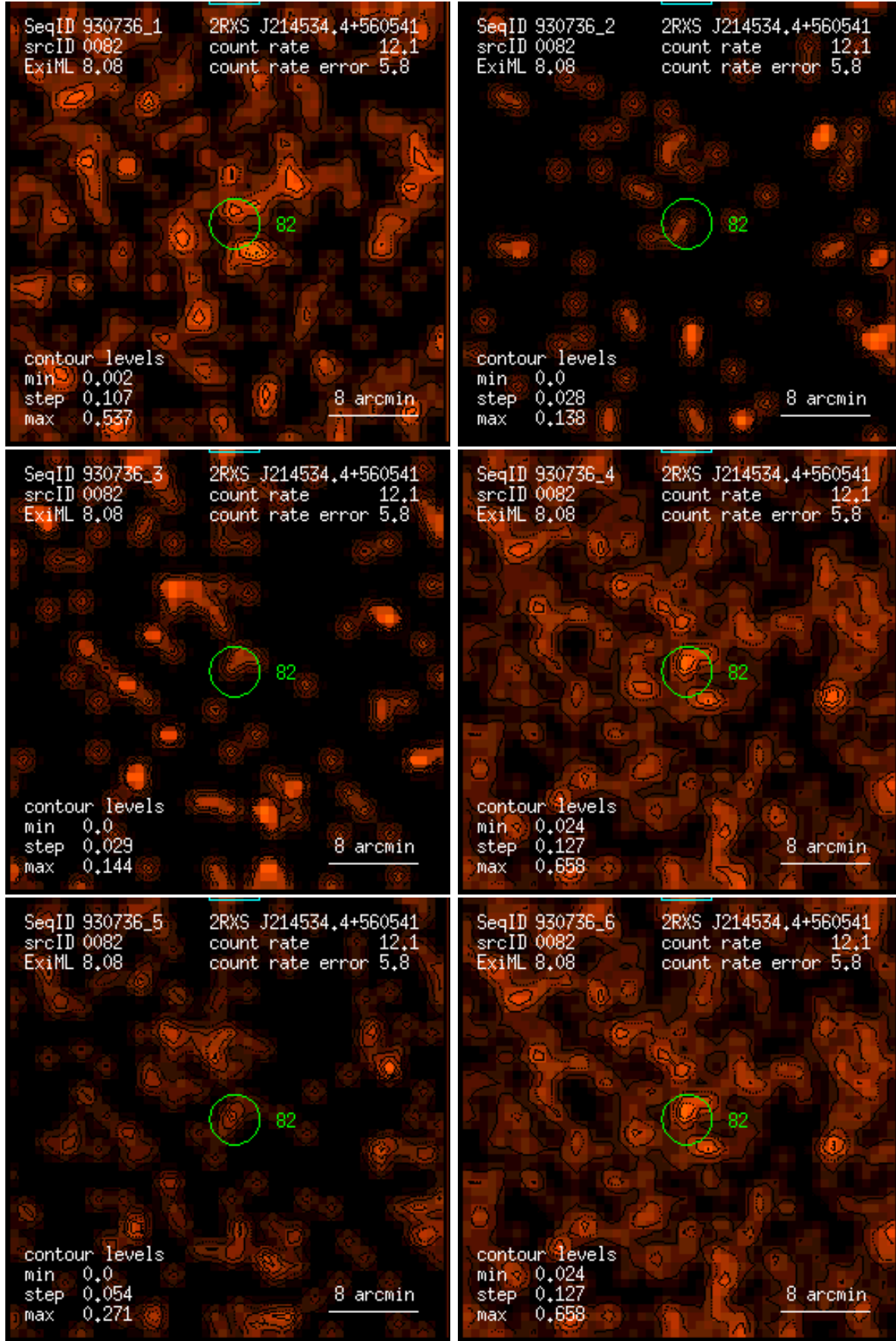
Figure 82: RASS 930736: detection 0082: band rate images, Gaussian filter: (1) PSPC channels 11 – 41, (2) 52 – 90, (3) 91 – 201, (4) 11 – 235, (5) 52 – 201, (6) 11 – 201. Broad band rates in counts/ks. Band rate contour levels in counts/ks/arcmin 2 .
