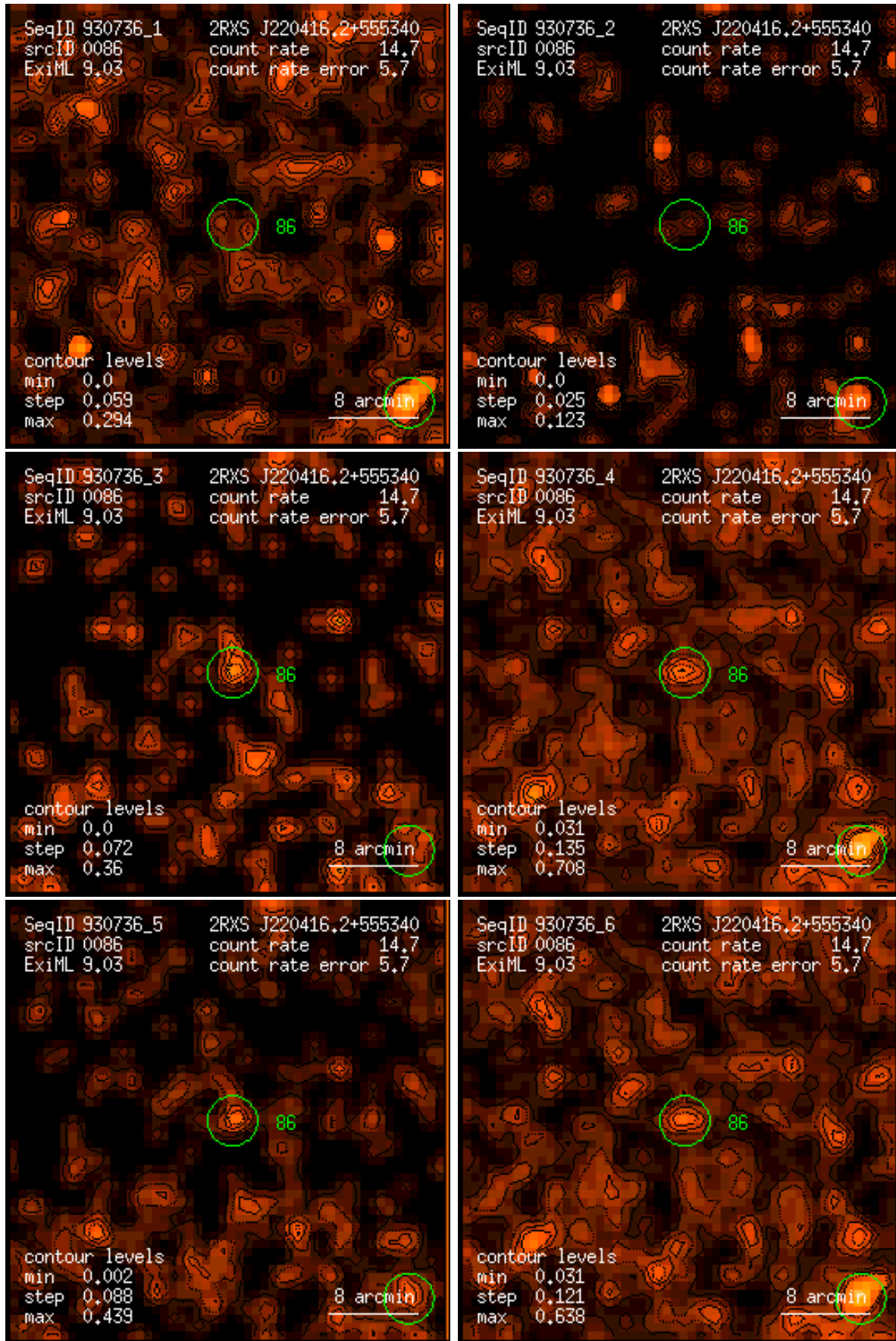
Figure 86: RASS 930736: detection 0086: band rate images, Gaussian filter: (1) PSPC channels 11 – 41, (2) 52 – 90, (3) 91 – 201, (4) 11 – 235, (5) 52 – 201, (6) 11 – 201. Broad band rates in counts/ks. Band rate contour levels in counts/ks/arcmin 2 .
