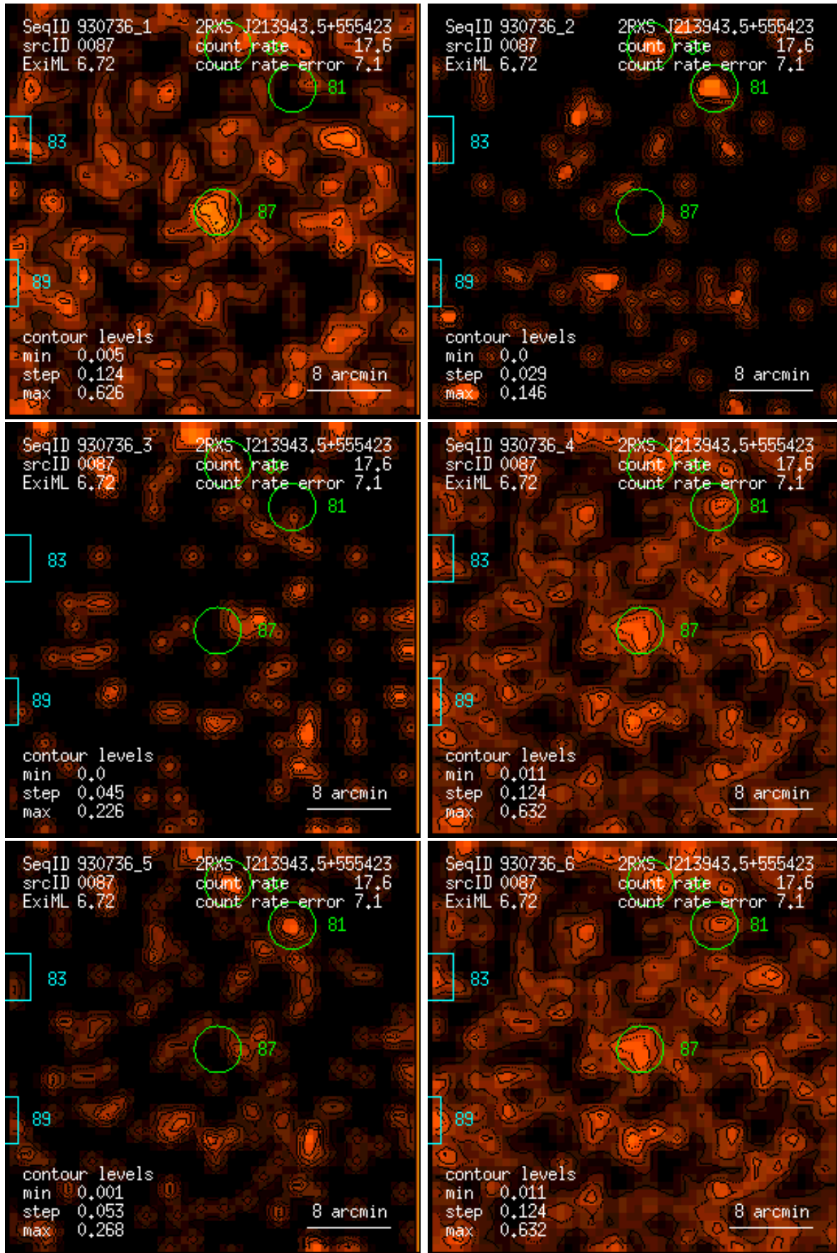
Figure 87: RASS 930736: detection 0087: band rate images, Gaussian filter: (1) PSPC channels 11 – 41, (2) 52 – 90, (3) 91 – 201, (4) 11 – 235, (5) 52 – 201, (6) 11 – 201. Broad band rates in counts/ks. Band rate contour levels in counts/ks/arcmin 2 .
