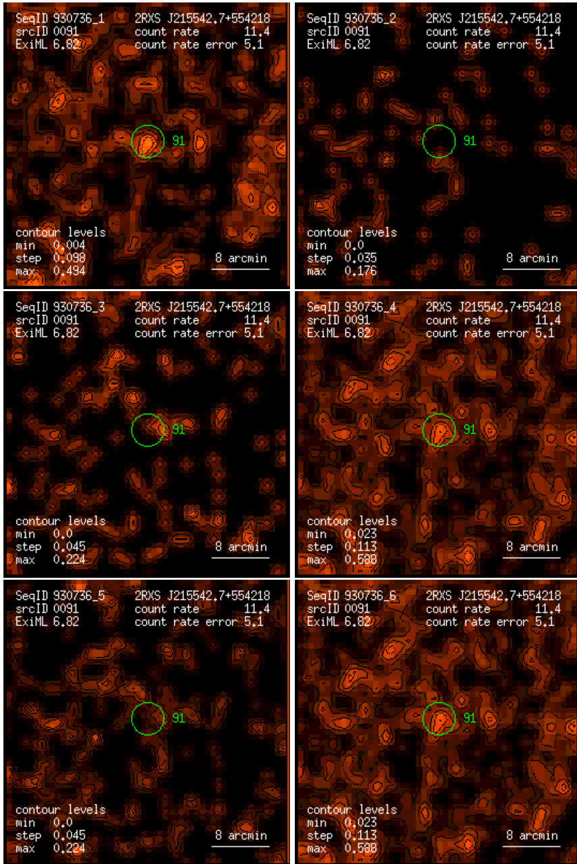
Figure 91: RASS 930736: detection 0091: band rate images, Gaussian filter: (1) PSPC channels 11 – 41, (2) 52 – 90, (3) 91 – 201, (4) 11 – 235, (5) 52 – 201, (6) 11 – 201. Broad band rates in counts/ks. Band rate contour levels in counts/ks/arcmin 2 .
