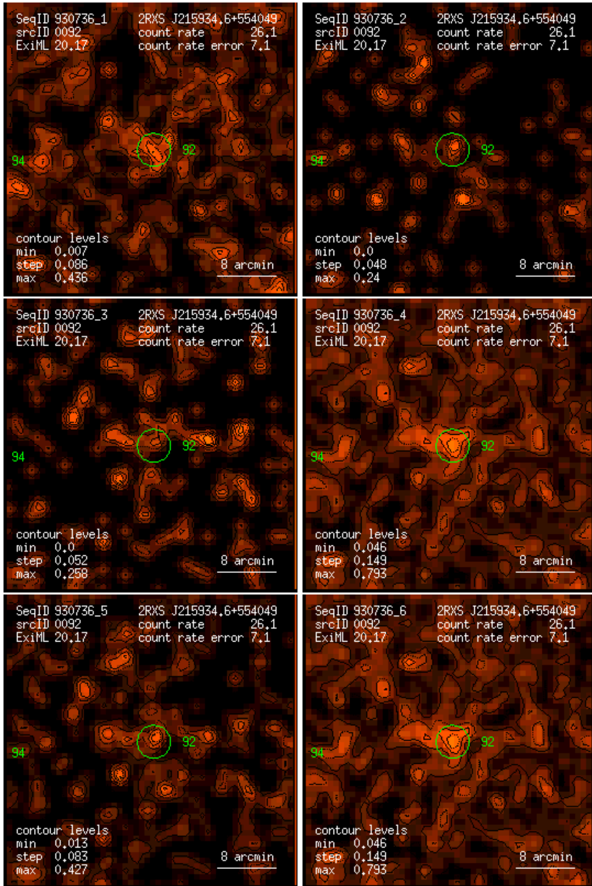
Figure 92: RASS 930736: detection 0092: band rate images, Gaussian filter: (1) PSPC channels 11 – 41, (2) 52 – 90, (3) 91 – 201, (4) 11 – 235, (5) 52 – 201, (6) 11 – 201. Broad band rates in counts/ks. Band rate contour levels in counts/ks/arcmin 2 .
