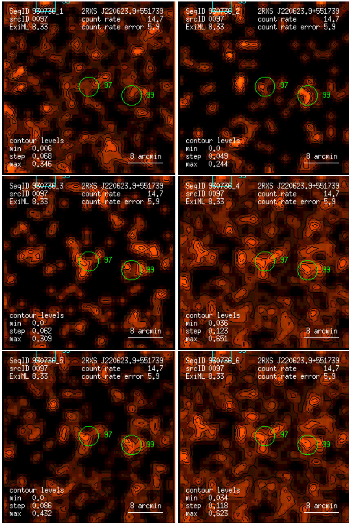
Figure 97: RASS 930736: detection 0097: band rate images, Gaussian filter: (1) PSPC channels 11 – 41, (2) 52 – 90, (3) 91 – 201, (4) 11 – 235, (5) 52 – 201, (6) 11 – 201. Broad band rates in counts/ks. Band rate contour levels in counts/ks/arcmin 2 .
