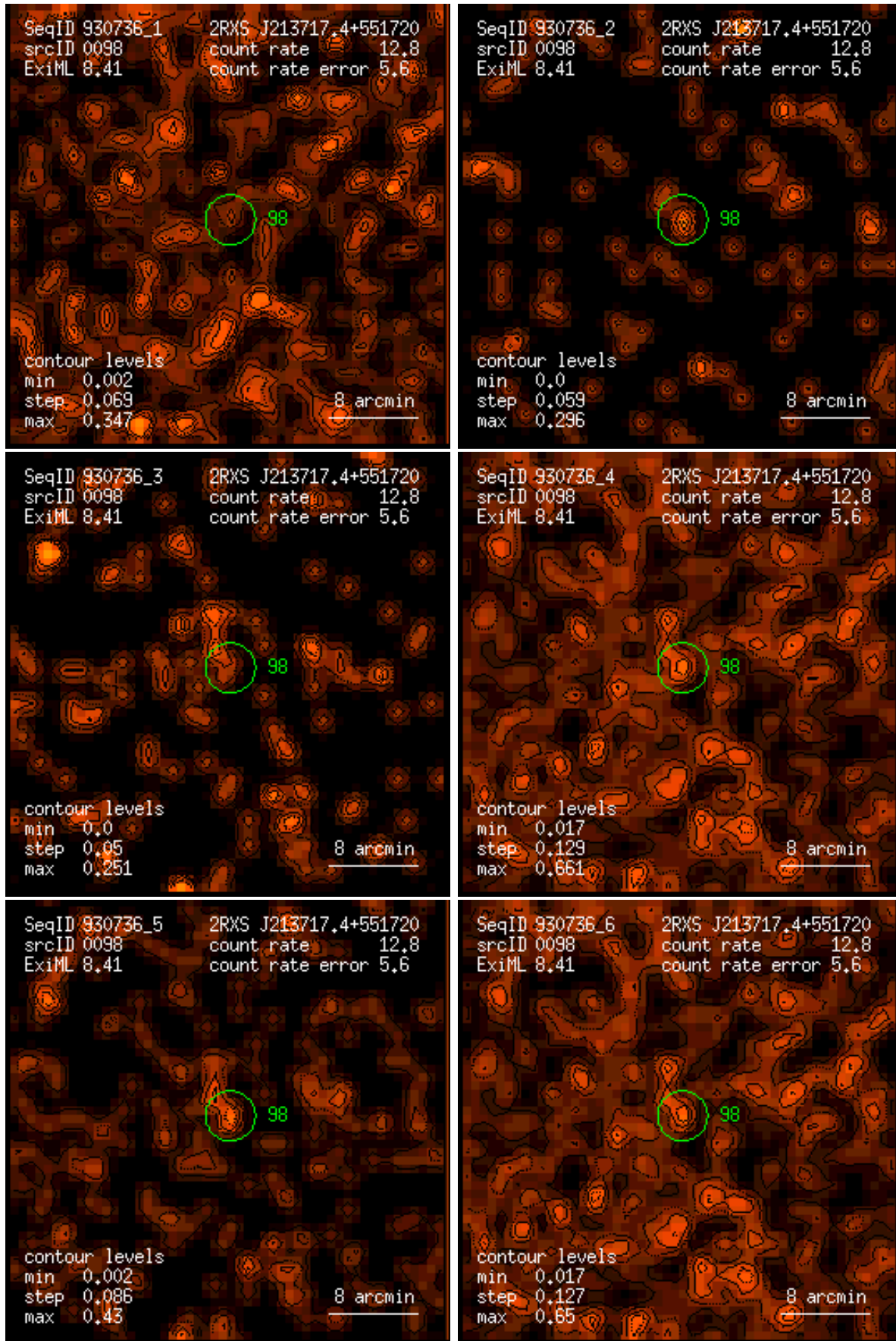
Figure 98: RASS 930736: detection 0098: band rate images, Gaussian filter: (1) PSPC channels 11 – 41, (2) 52 – 90, (3) 91 – 201, (4) 11 – 235, (5) 52 – 201, (6) 11 – 201. Broad band rates in counts/ks. Band rate contour levels in counts/ks/arcmin 2 .
