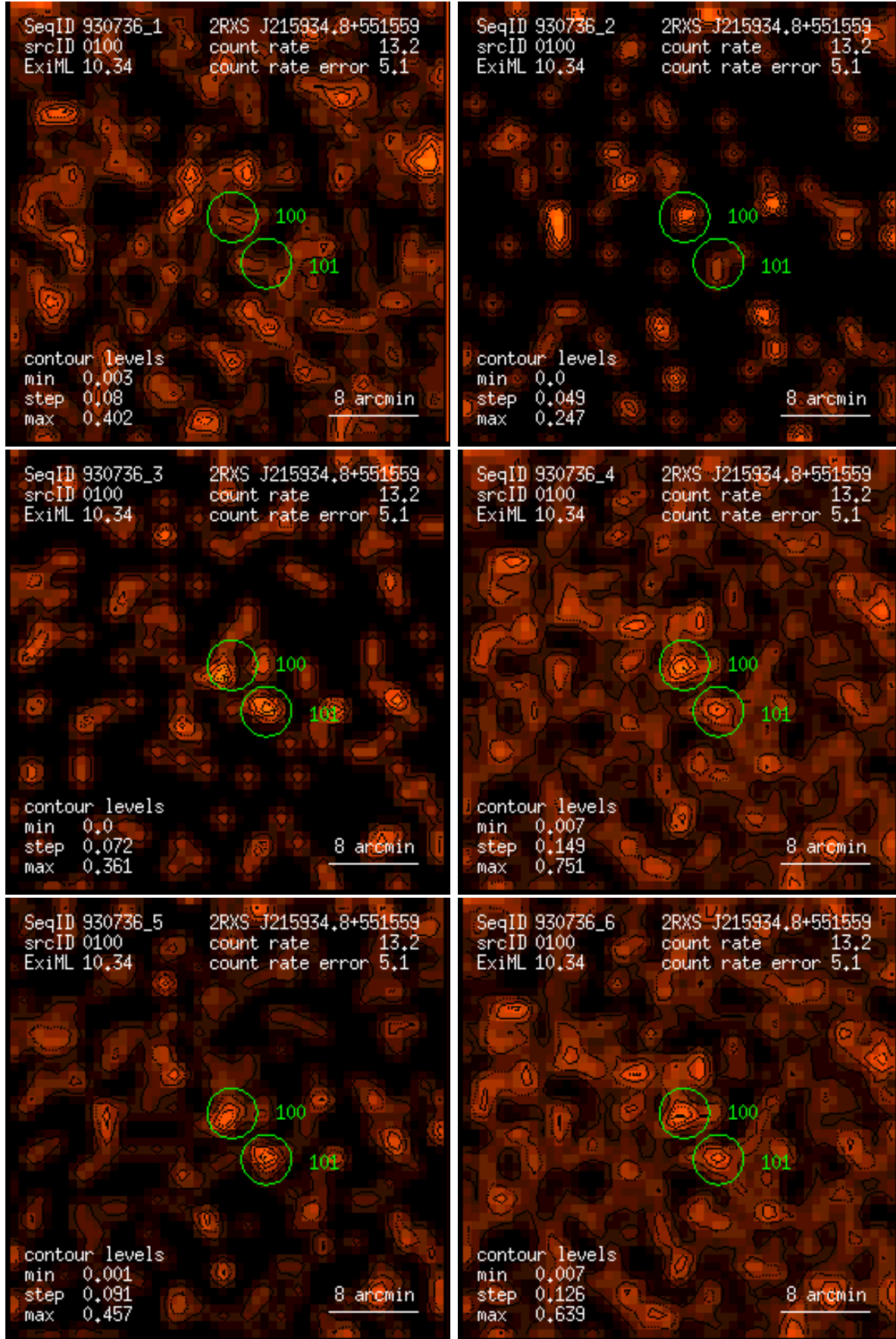
Figure 100: RASS 930736: detection 0100: band rate images, Gaussian filter: (1) PSPC channels 11 – 41, (2) 52 – 90, (3) 91 – 201, (4) 11 – 235, (5) 52 – 201, (6) 11 – 201. Broad band rates in counts/ks. Band rate contour levels in counts/ks/arcmin 2 .
