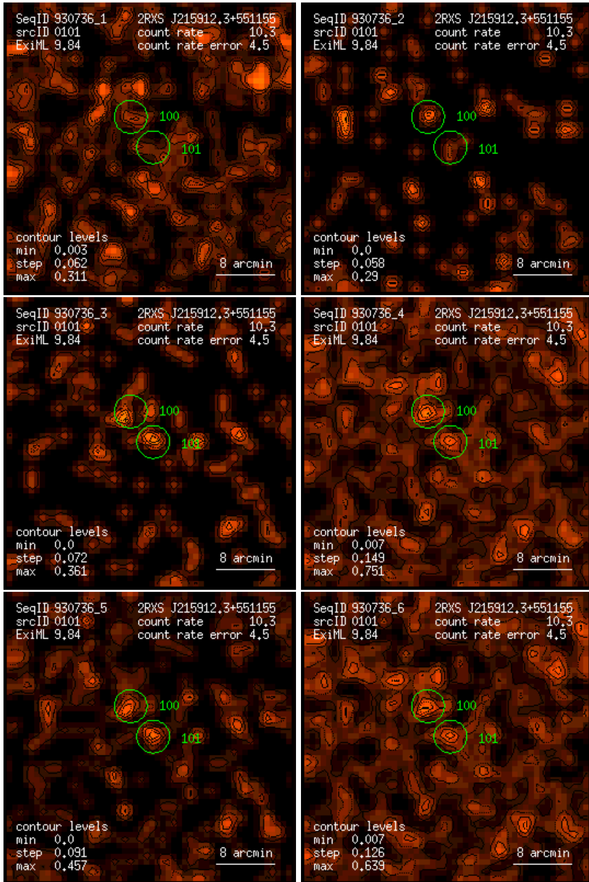
Figure 101: RASS 930736: detection 0101: band rate images, Gaussian filter: (1) PSPC channels 11 – 41, (2) 52 – 90, (3) 91 – 201, (4) 11 – 235, (5) 52 – 201, (6) 11 – 201. Broad band rates in counts/ks. Band rate contour levels in counts/ks/arcmin 2 .
