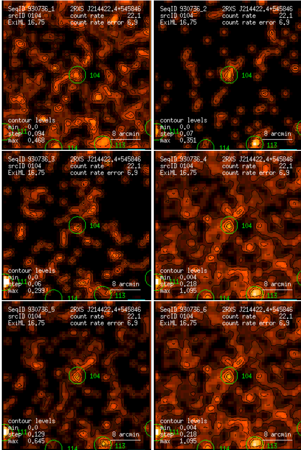
Figure 104: RASS 930736: detection 0104: band rate images, Gaussian filter: (1) PSPC channels 11 – 41, (2) 52 – 90, (3) 91 – 201, (4) 11 – 235, (5) 52 – 201, (6) 11 – 201. Broad band rates in counts/ks. Band rate contour levels in counts/ks/arcmin 2 .
