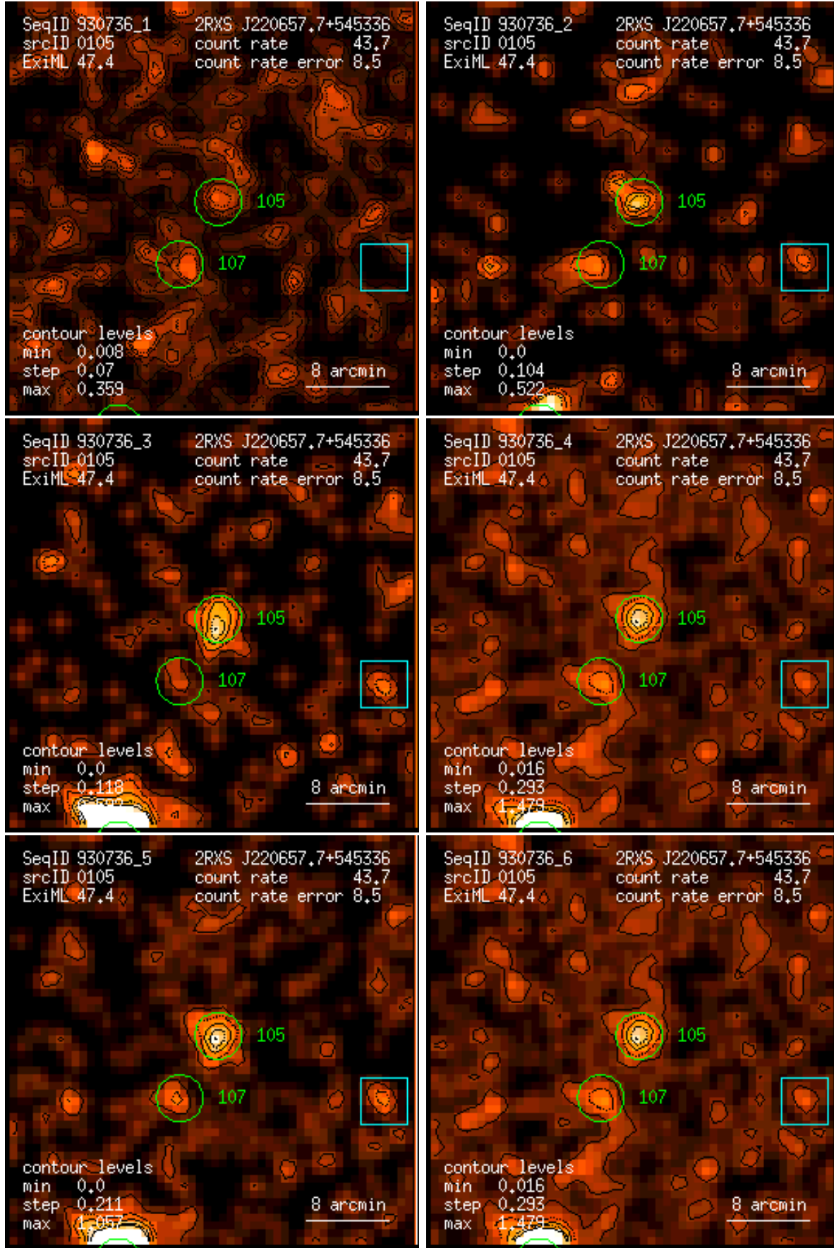
Figure 105: RASS 930736: detection 0105: band rate images, Gaussian filter: (1) PSPC channels 11 – 41, (2) 52 – 90, (3) 91 – 201, (4) 11 – 235, (5) 52 – 201, (6) 11 – 201. Broad band rates in counts/ks. Band rate contour levels in counts/ks/arcmin 2 .
