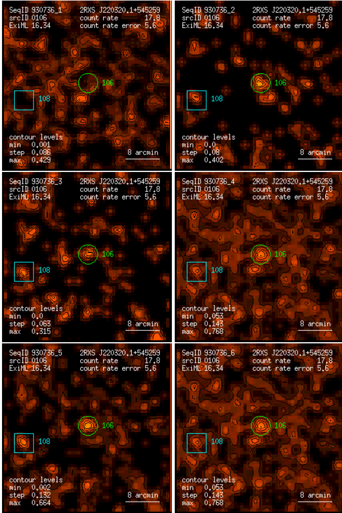
Figure 106: RASS 930736: detection 0106: band rate images, Gaussian filter: (1) PSPC channels 11 – 41, (2) 52 – 90, (3) 91 – 201, (4) 11 – 235, (5) 52 – 201, (6) 11 – 201. Broad band rates in counts/ks. Band rate contour levels in counts/ks/arcmin 2 .
