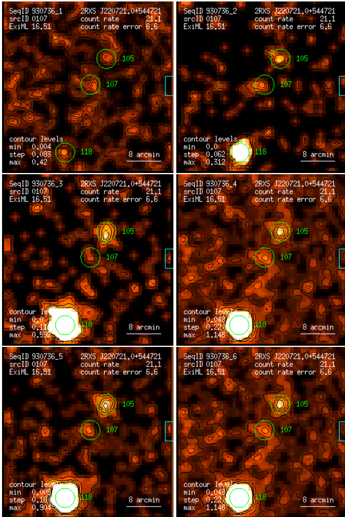
Figure 107: RASS 930736: detection 0107: band rate images, Gaussian filter: (1) PSPC channels 11 – 41, (2) 52 – 90, (3) 91 – 201, (4) 11 – 235, (5) 52 – 201, (6) 11 – 201. Broad band rates in counts/ks. Band rate contour levels in counts/ks/arcmin 2 .
