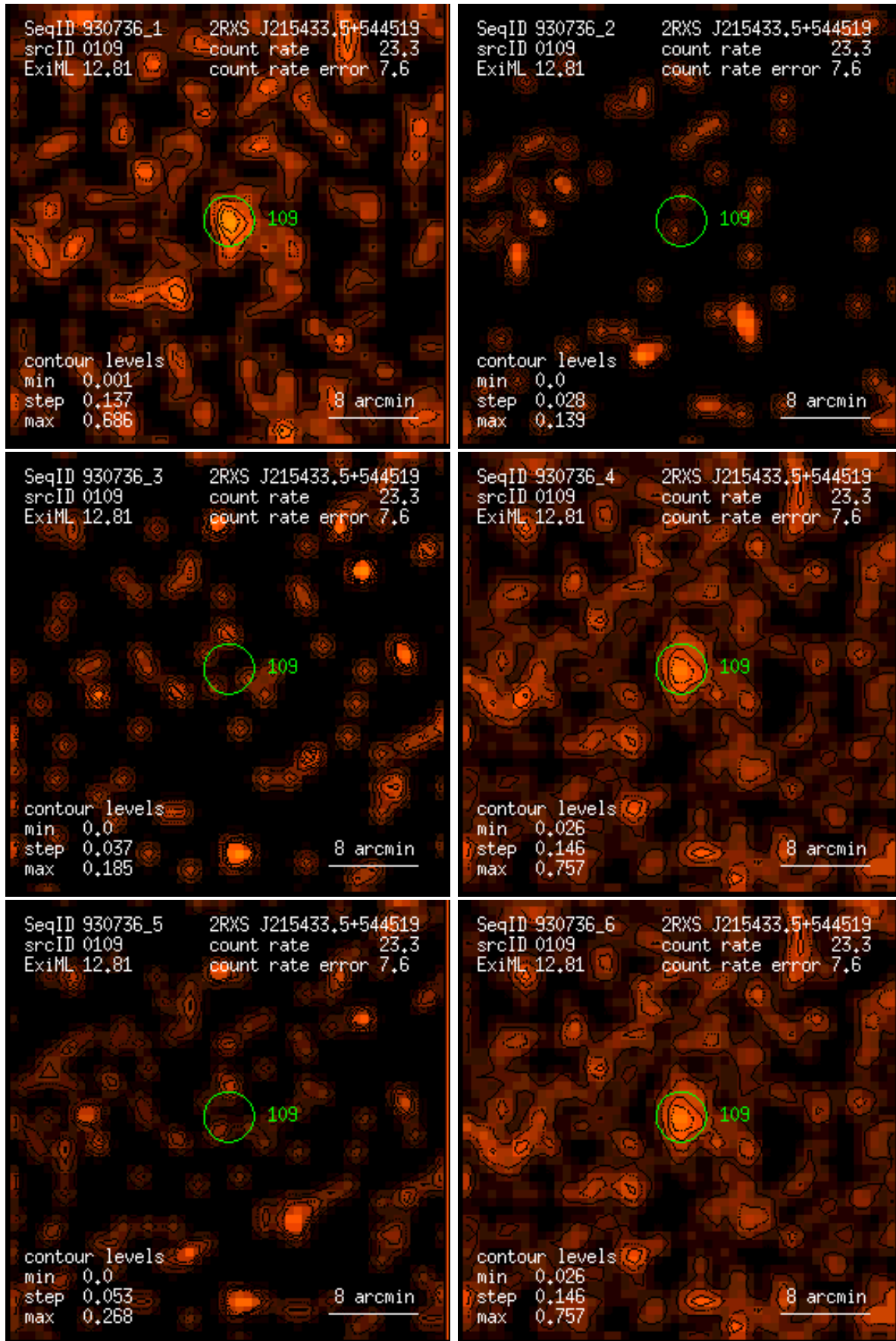
Figure 109: RASS 930736: detection 0109: band rate images, Gaussian filter: (1) PSPC channels 11 – 41, (2) 52 – 90, (3) 91 – 201, (4) 11 – 235, (5) 52 – 201, (6) 11 – 201. Broad band rates in counts/ks. Band rate contour levels in counts/ks/arcmin 2 .
