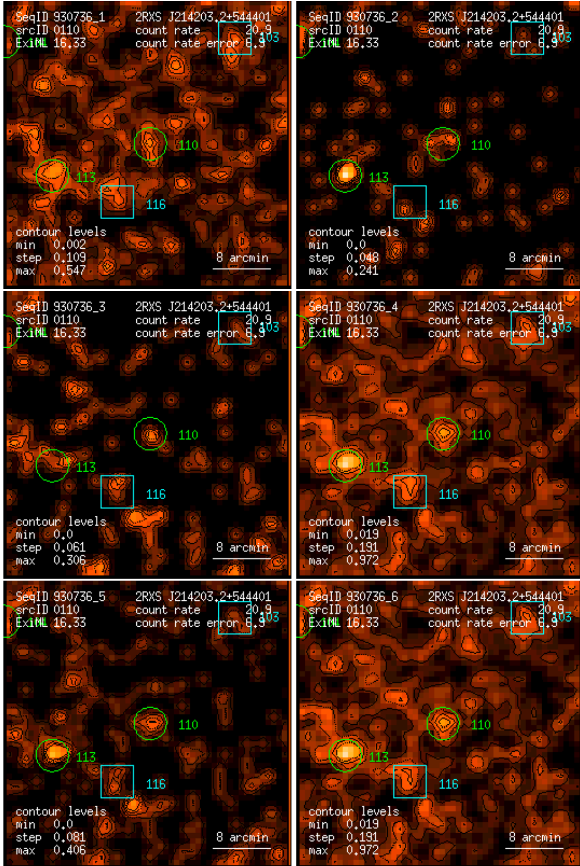
Figure 110: RASS 930736: detection 0110: band rate images, Gaussian filter: (1) PSPC channels 11 – 41, (2) 52 – 90, (3) 91 – 201, (4) 11 – 235, (5) 52 – 201, (6) 11 – 201. Broad band rates in counts/ks. Band rate contour levels in counts/ks/arcmin 2 .
