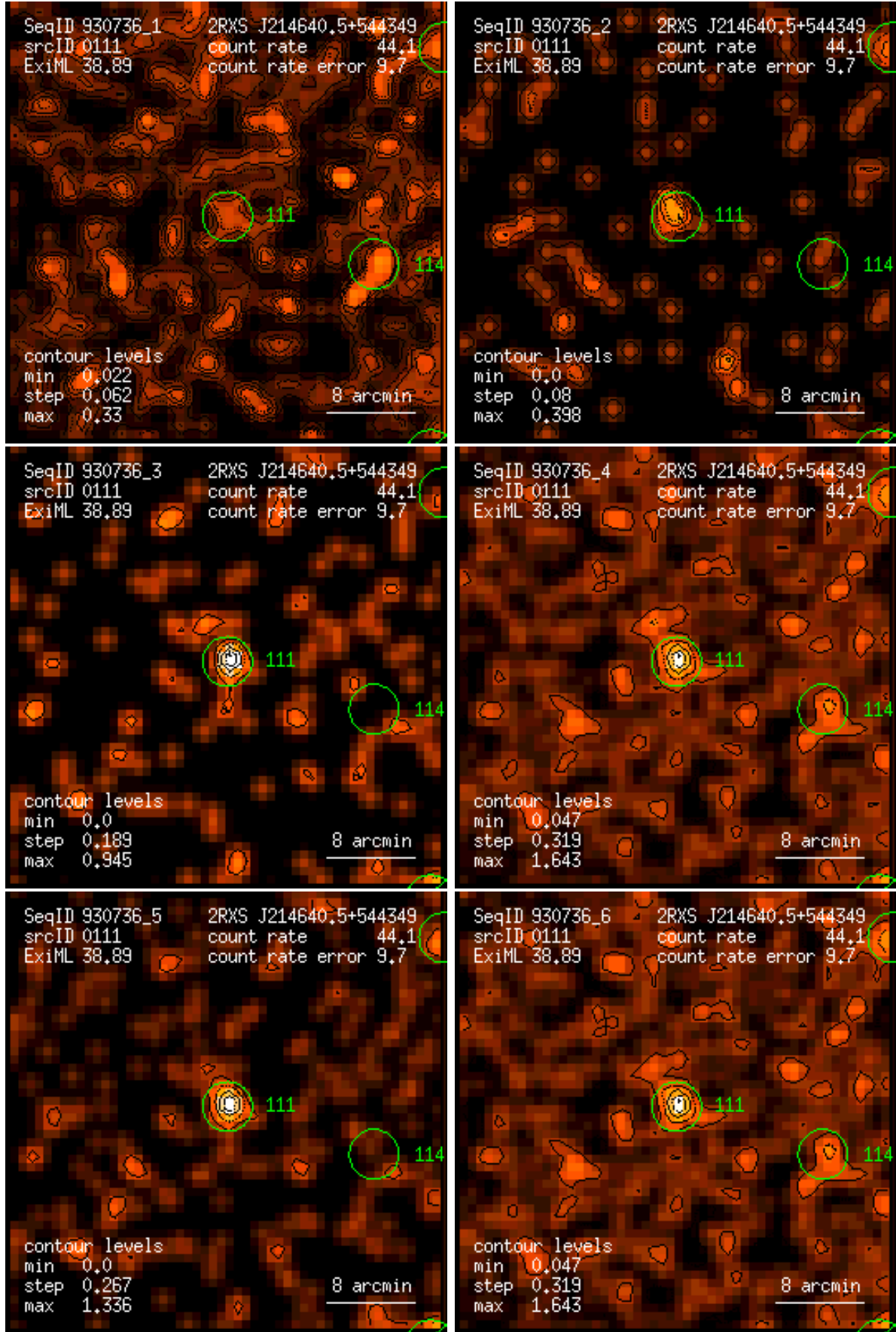
Figure 111: RASS 930736: detection 0111: band rate images, Gaussian filter: (1) PSPC channels 11 – 41, (2) 52 – 90, (3) 91 – 201, (4) 11 – 235, (5) 52 – 201, (6) 11 – 201. Broad band rates in counts/ks. Band rate contour levels in counts/ks/arcmin 2 .
