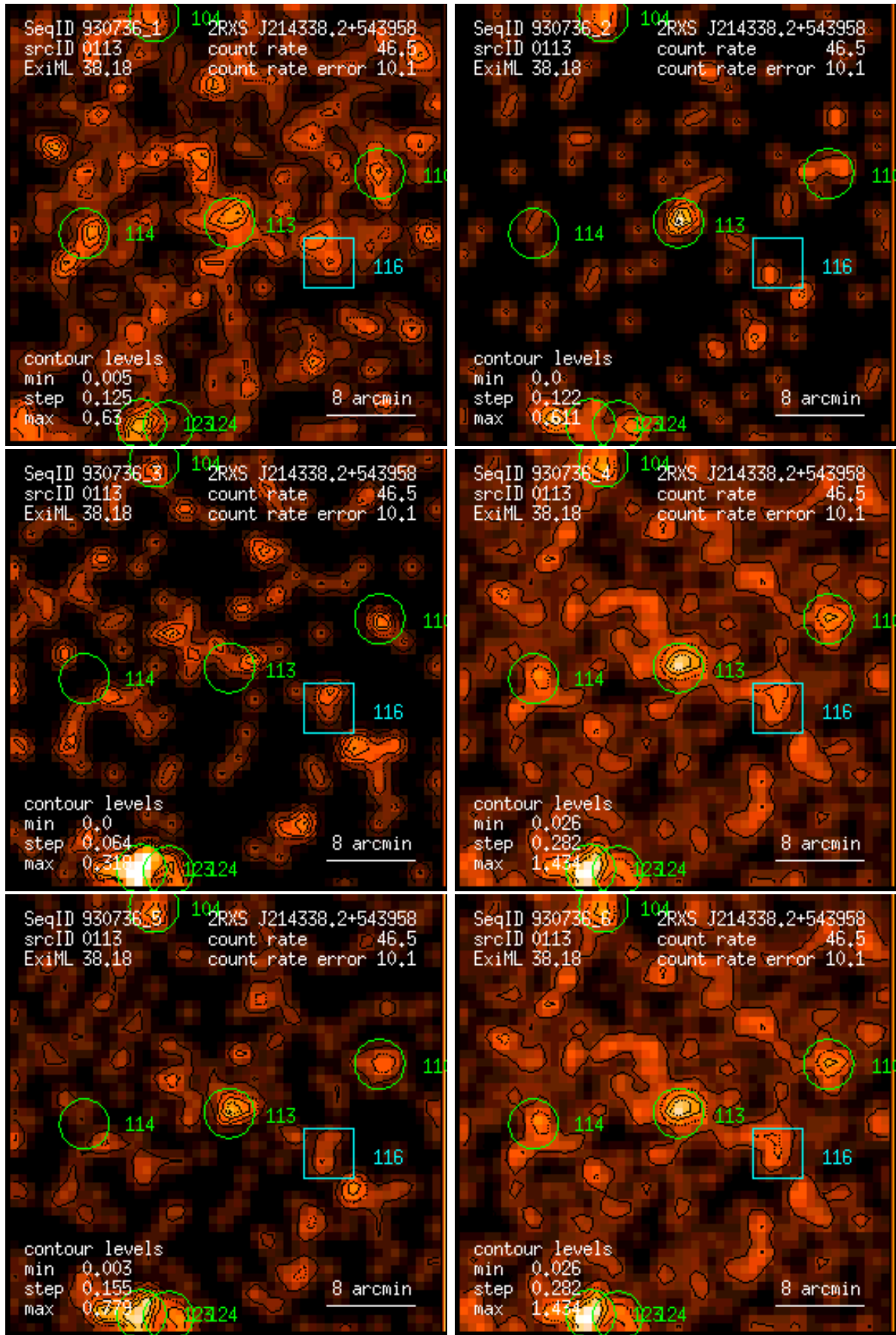
Figure 113: RASS 930736: detection 0113: band rate images, Gaussian filter: (1) PSPC channels 11 – 41, (2) 52 – 90, (3) 91 – 201, (4) 11 – 235, (5) 52 – 201, (6) 11 – 201. Broad band rates in counts/ks. Band rate contour levels in counts/ks/arcmin 2 .
