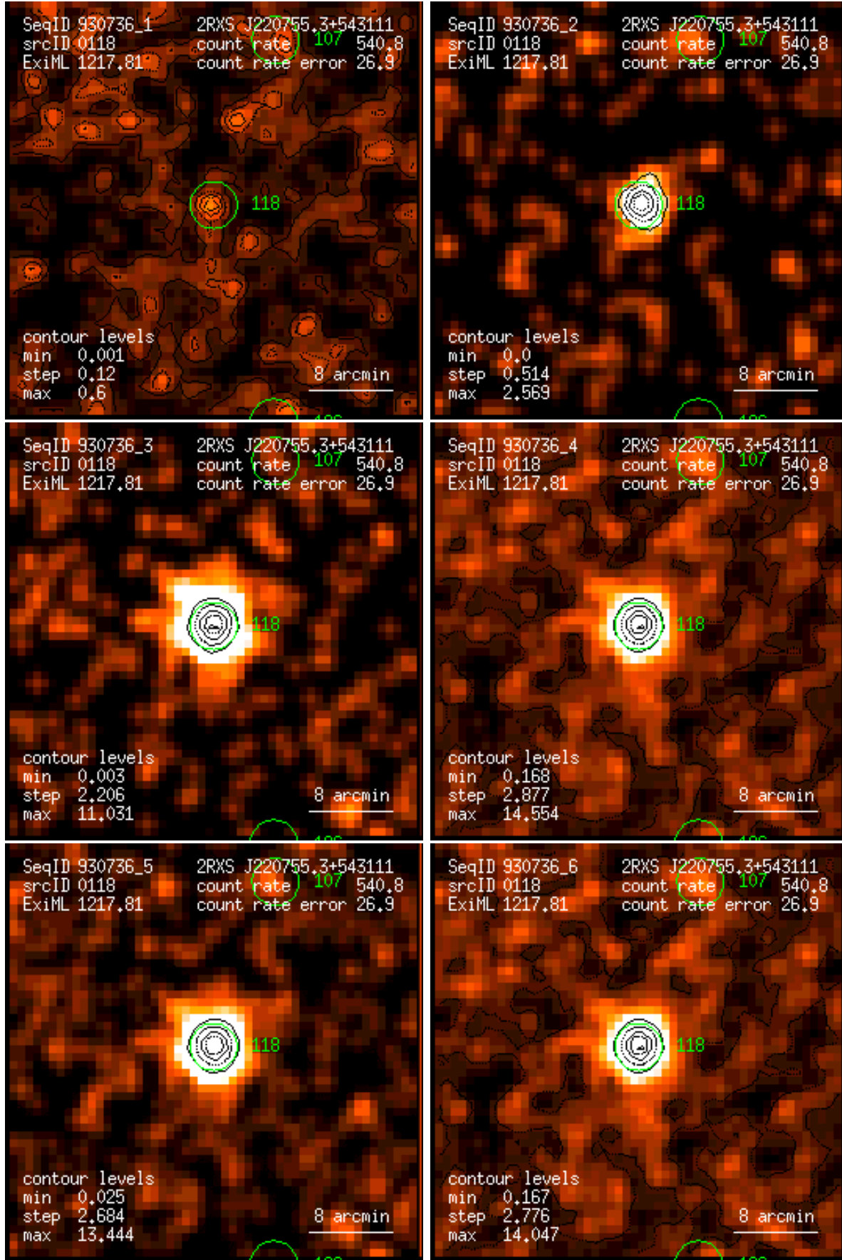
Figure 118: RASS 930736: detection 0118: band rate images, Gaussian filter: (1) PSPC channels 11 – 41, (2) 52 – 90, (3) 91 – 201, (4) 11 – 235, (5) 52 – 201, (6) 11 – 201. Broad band rates in counts/ks. Band rate contour levels in counts/ks/arcmin 2 .
